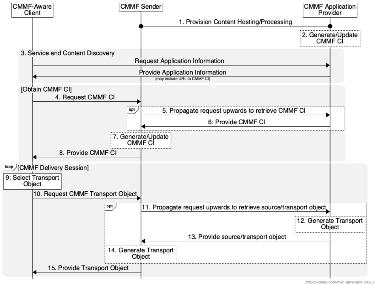
Figure D.5: High-level procedure for URL translation-based CMMF provisioning and preparation
