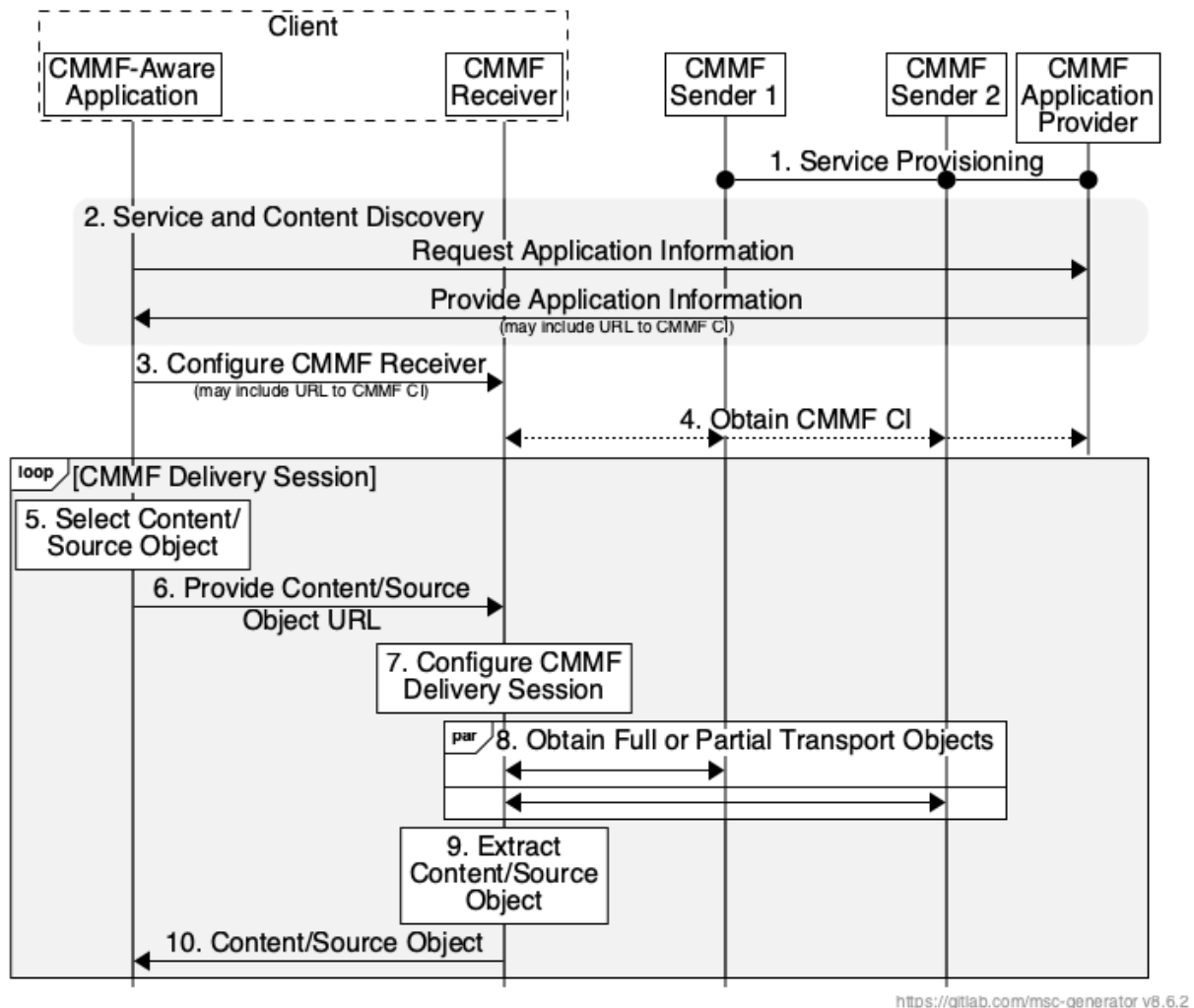
Figure D.6: High-level procedure for URL Translation-based CMMF CDP delivery
