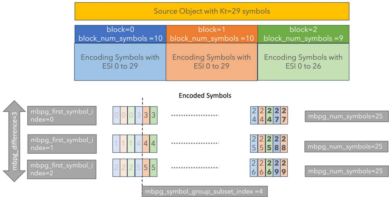
Figure 13: Example symbol arrangement for mbpg_symbol_arrangement=0011b (Encoded-Symbol Interleaved Arrangement)
