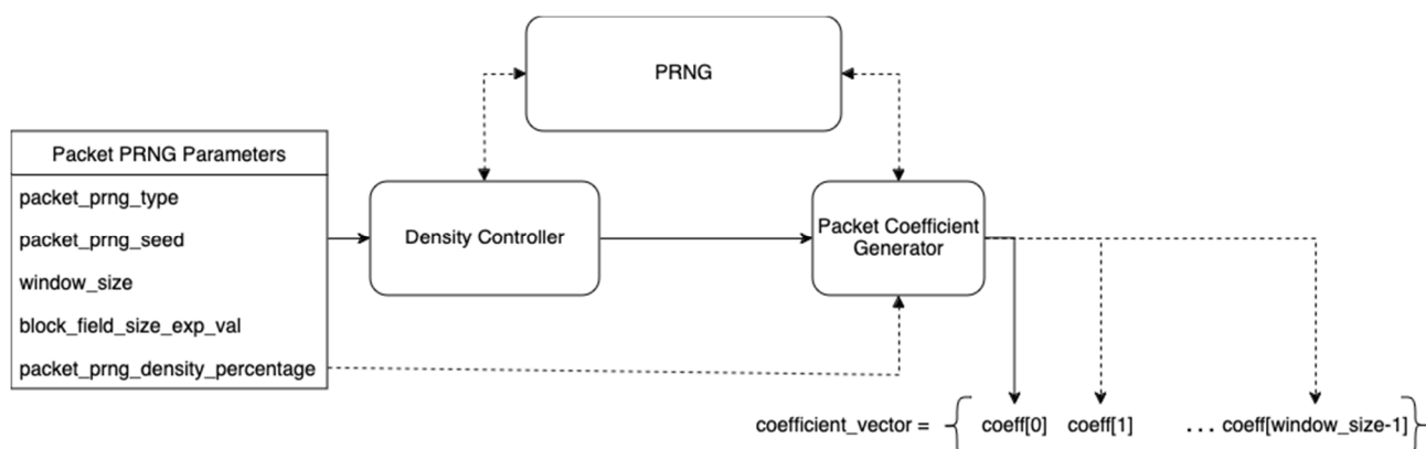
Figure 15: Packet PRNG
