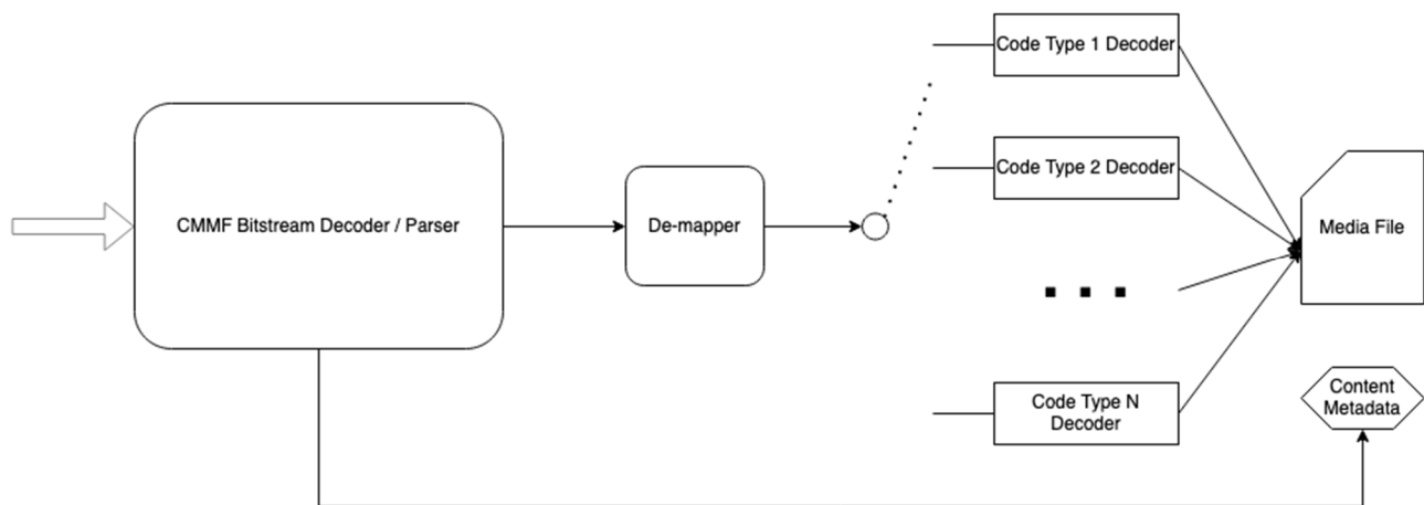
Figure 6: CMMF bitstream decoding
