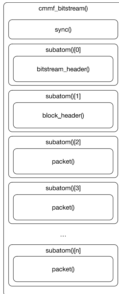
Figure F.1: CMMF bitstream layout for CMMF bitstream profile A
