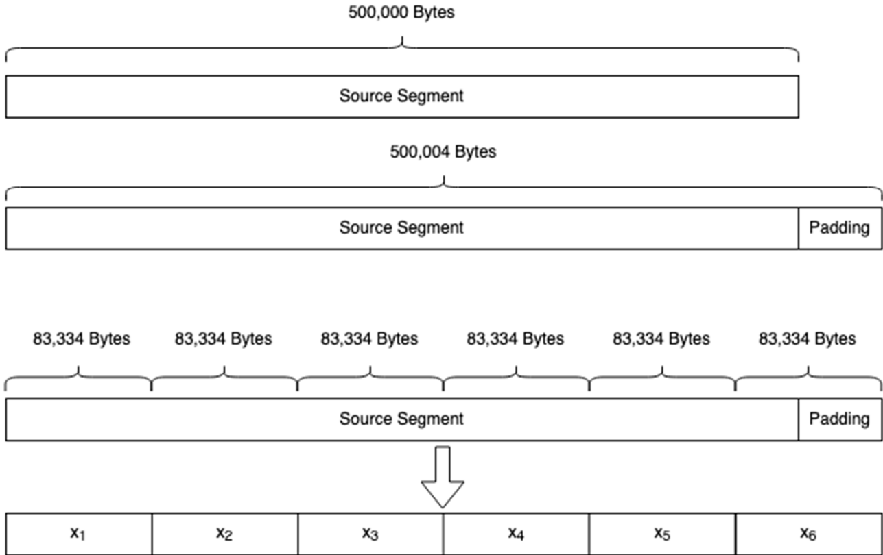
Figure A.1: xCD-1 segment to symbols
