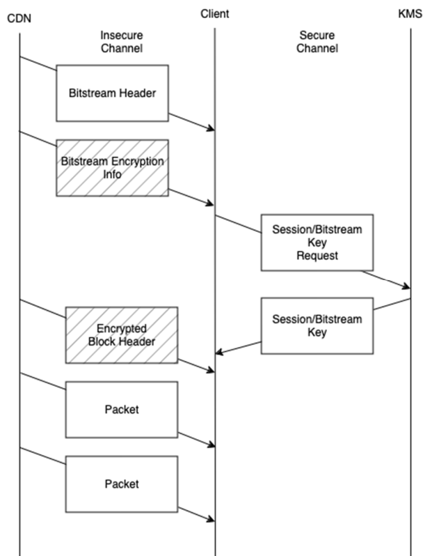
Figure 19: Bitstream and key download process
