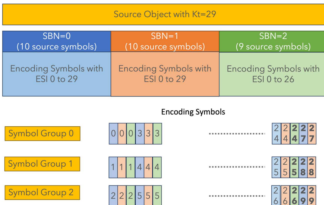
Figure D.3: Symbol arrangement for arrangement 3
