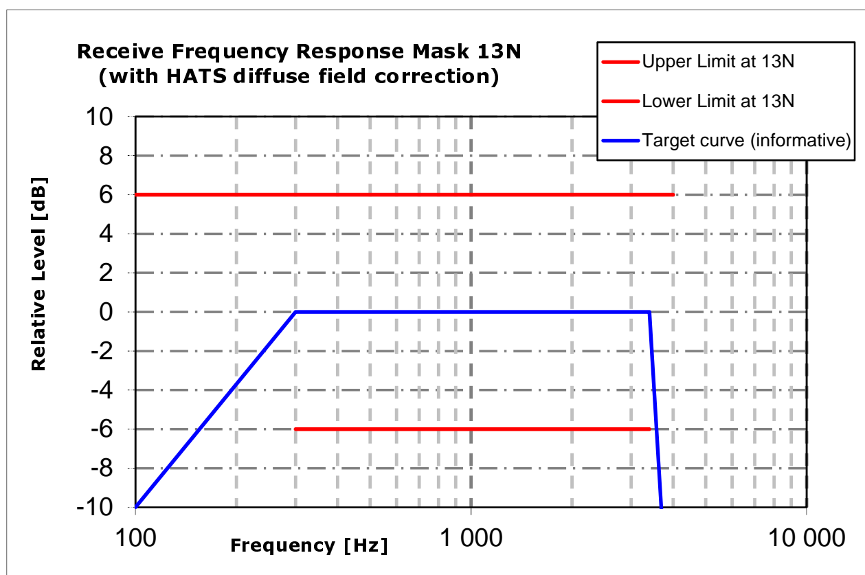
Figure 6.1.2.2: Receive frequency response mask for 13N application force
