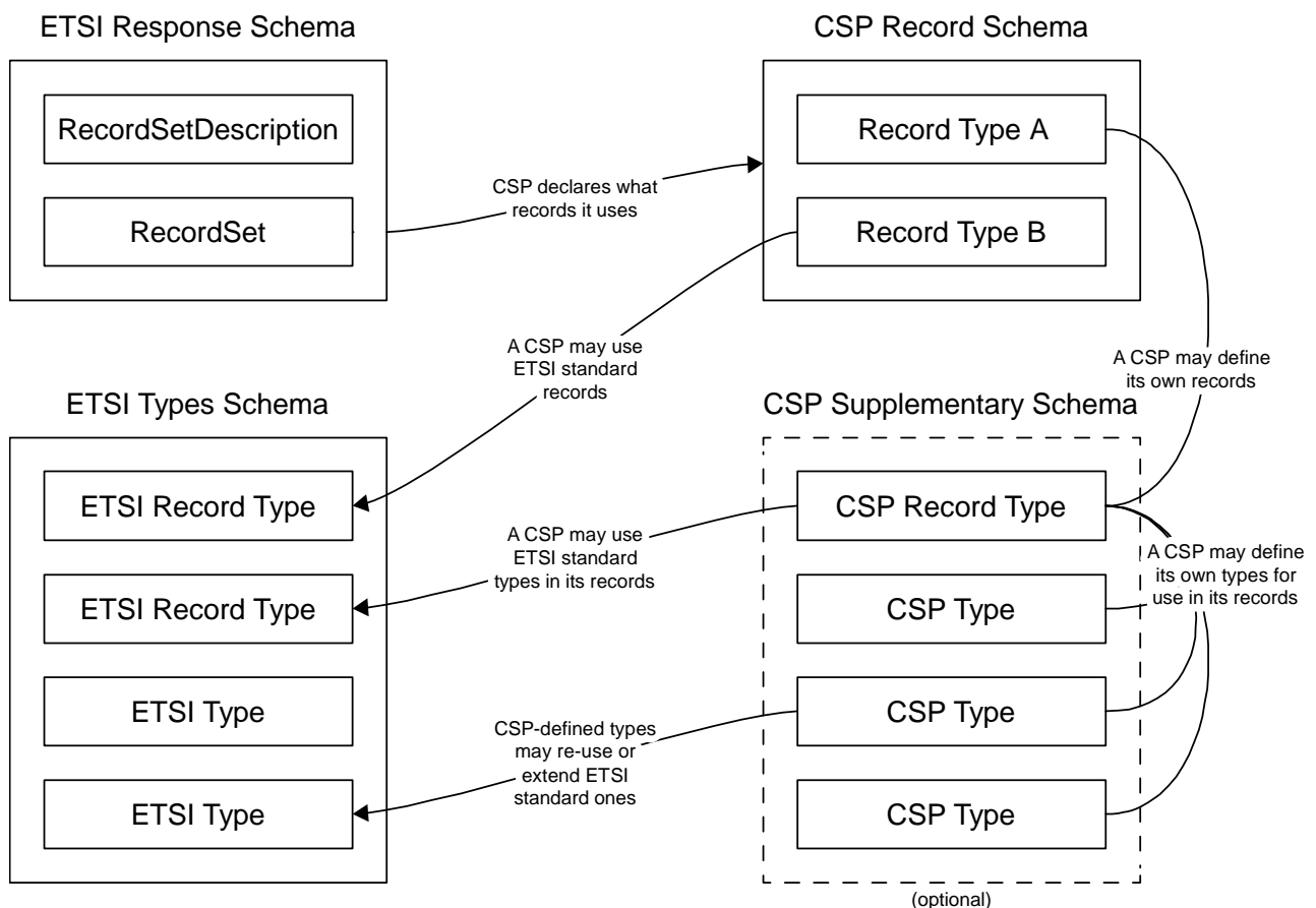
Figure 6.1-1: JSON schema structure
