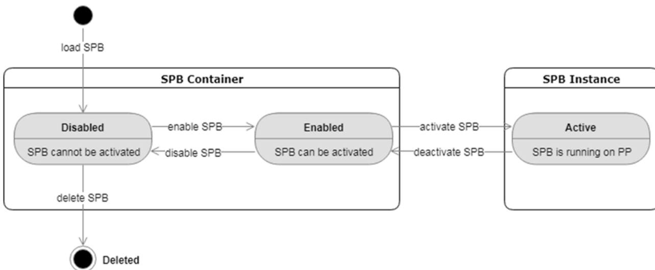
Figure 9.1: Secondary Platform Bundle states
