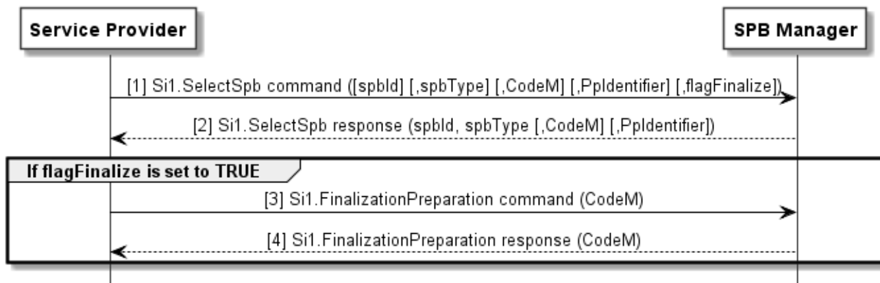
Figure 12.4: Secondary Platform Bundle selection process
