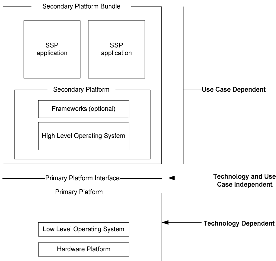
Figure 6.1: iSSP architecture
