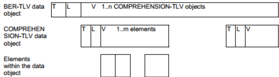
Figure 10.9: Data objects
