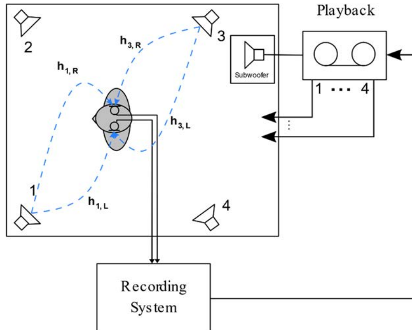
Figure 24: Binaural noise field simulation
