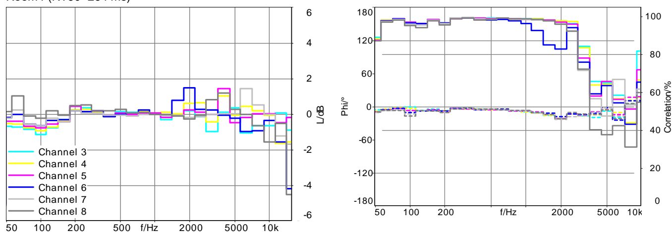
Figure 13: Level difference between reference and simulated sound field as well as the complex coherence in magnitude (solid) and phase(dashed)
