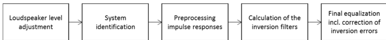
Figure 6: Blocks of the equalization procedure
