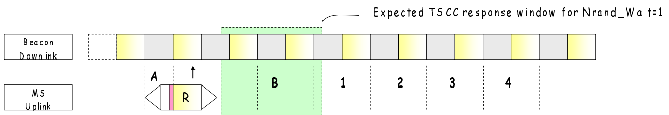
Figure 12.19: Random backoff Example #2
