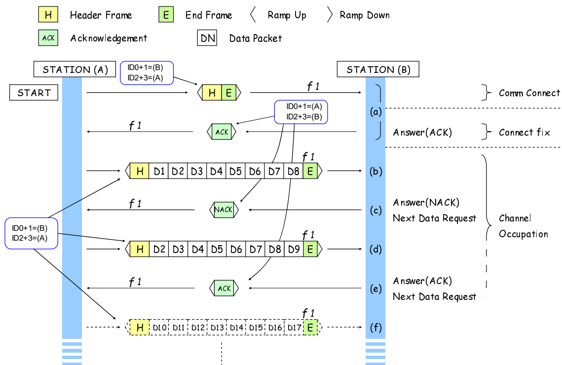
Figure 10.7: Packet Retransmissions
