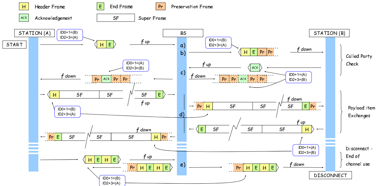
Figure 4.23: Mode 2 Voice Call Example
