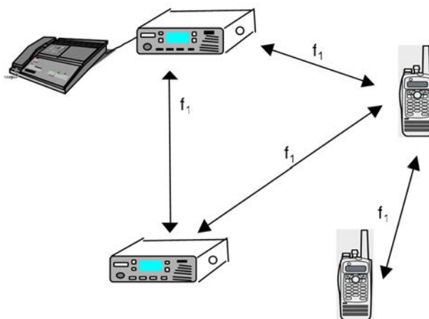
Figure 4.2: Peer-to-Peer Direct Network (Mode 1)
