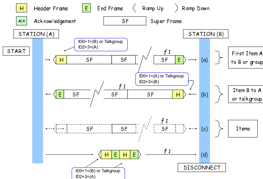
Figure 4.20: Mode 1 voice call message exchange
