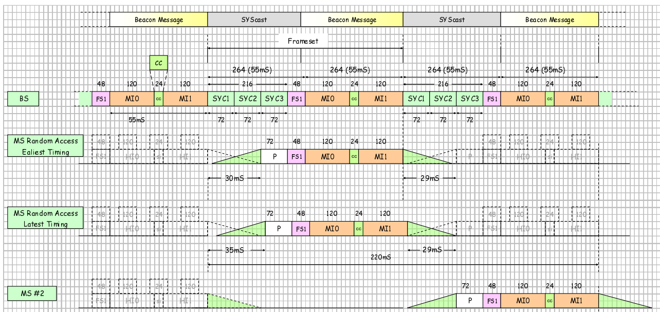
Figure 12.7: Beacon Timing
