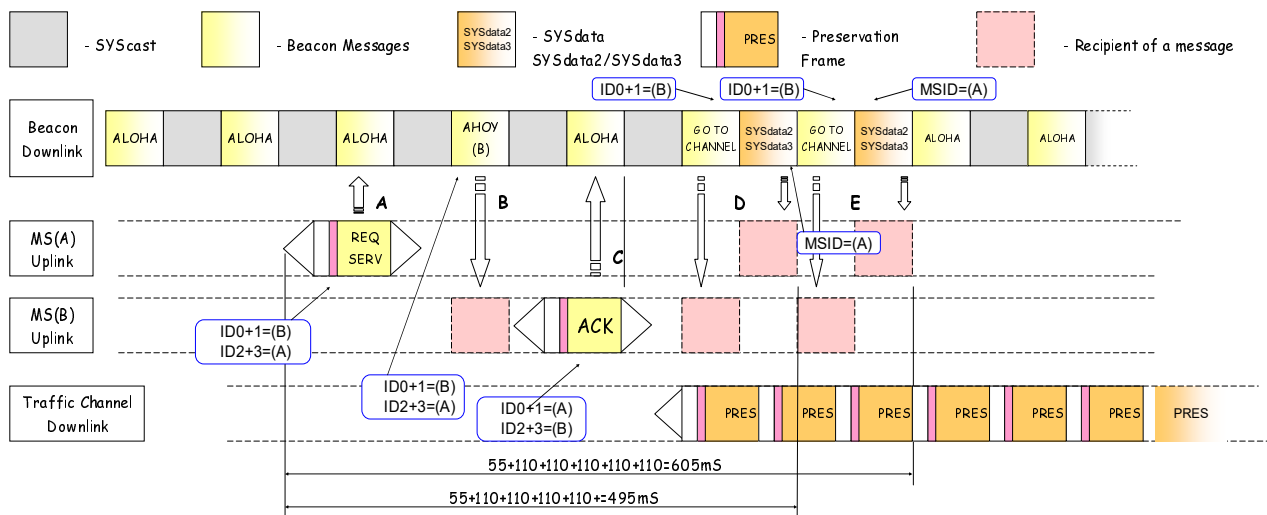
Figure 10.27: Individual Call Set-up example
