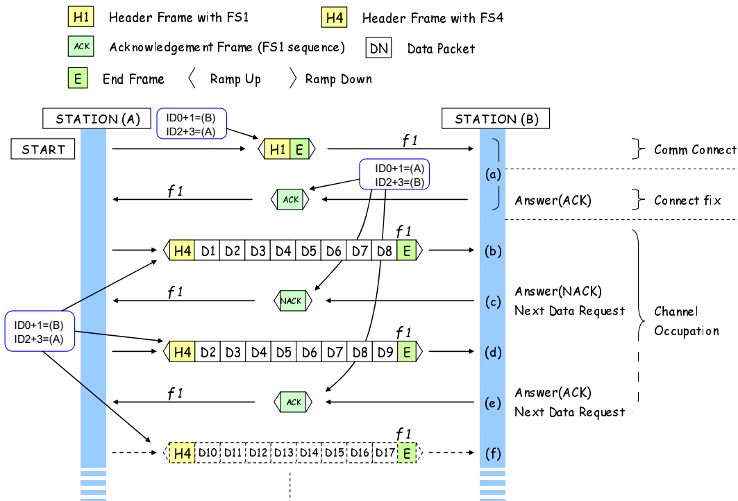
Figure 9.4: Packet retransmissions
