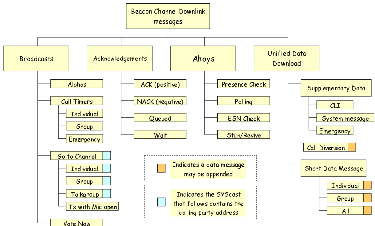
Figure 8.3: Downlink Beacon Messages
