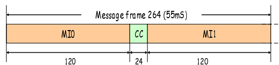
Figure 4.6: Beacon Channel Message Frame
