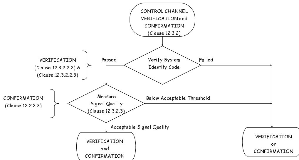
Figure 12.26: Verification and Confirmation Steps
