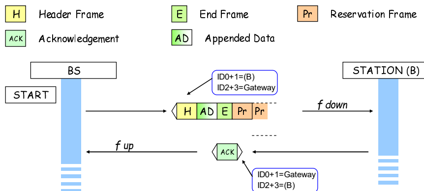
Figure 10.22: Call from a line connected source
