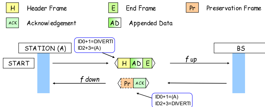
Figure 10.18: Call Diversion
