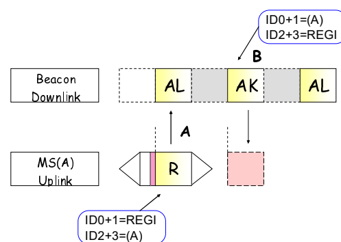
Figure 12.31: Registration Exchange
