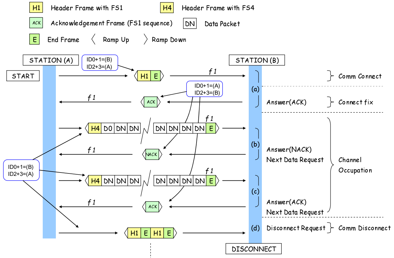
Figure 9.3: Packet exchanges
