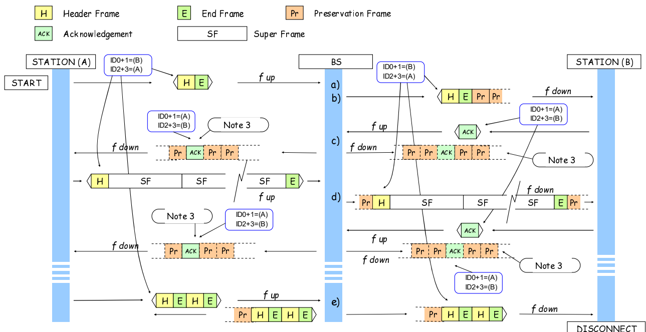
Figure 10.15: Mode 2 Individual data call exchanges
