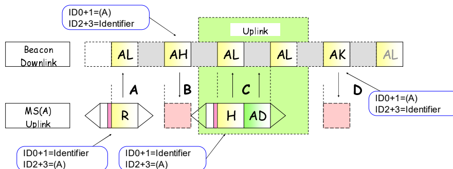
Figure 10.42: Example of a Call Diversion Call
