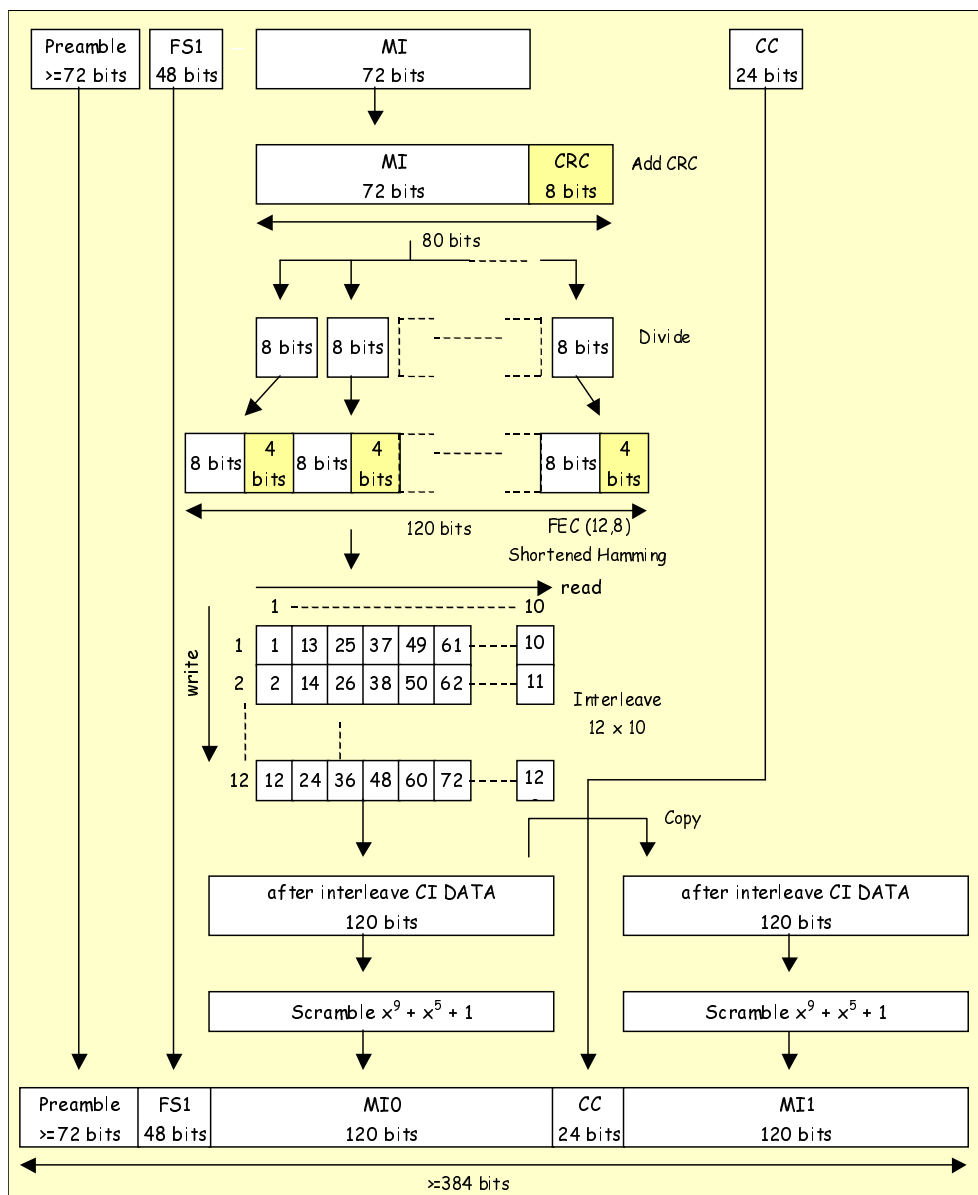
Figure 11.8: Message coding
