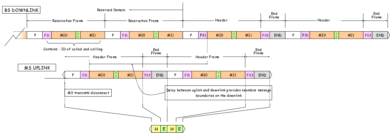
Figure 10.14: End of the call
