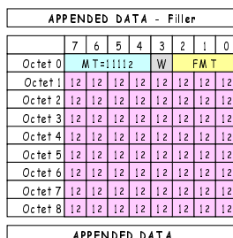
Figure 5.17: Appended_Data Filler
