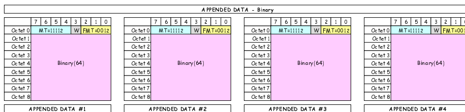
Figure 5.10: Appended_Data (Binary)
