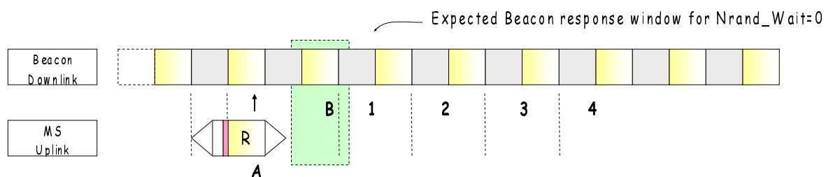
Figure 12.18: Random Backoff Example #1
