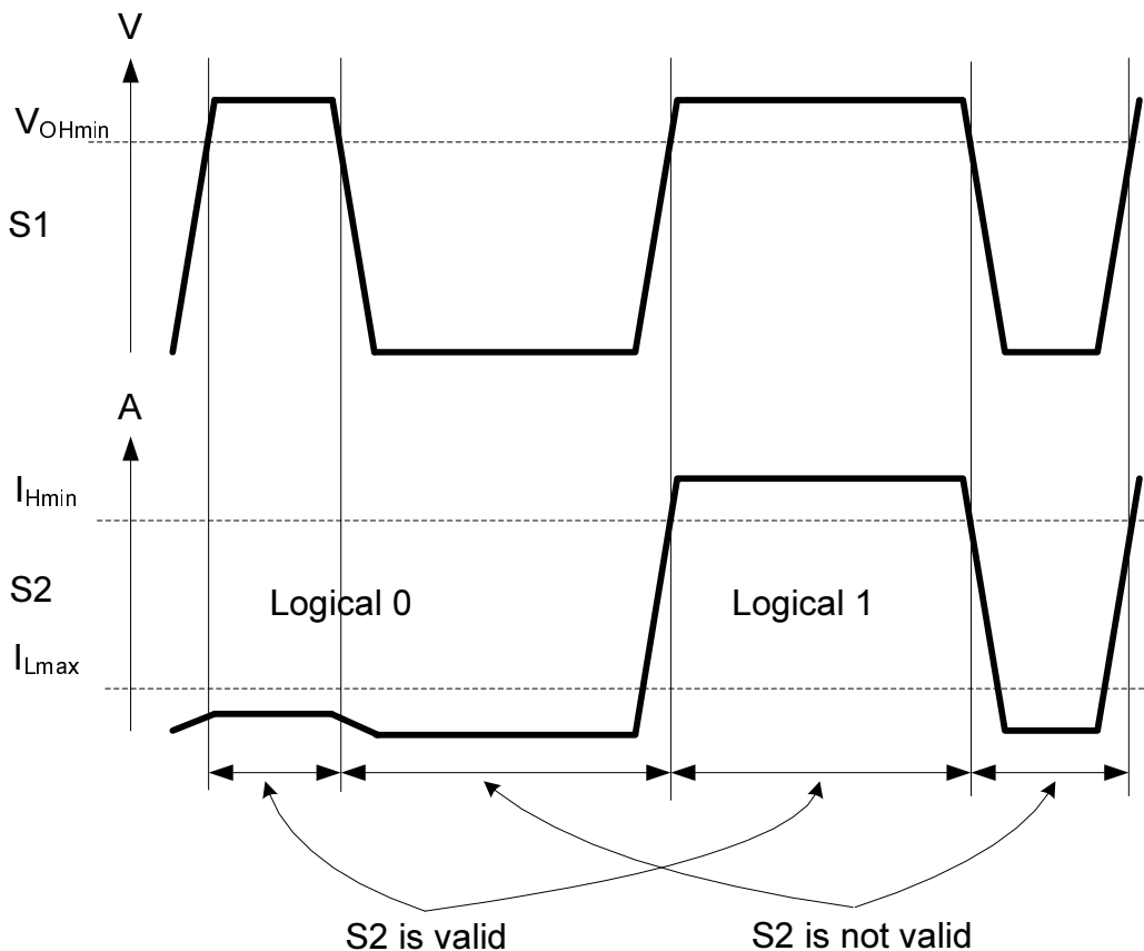
Figure 8.3: S2 timing
