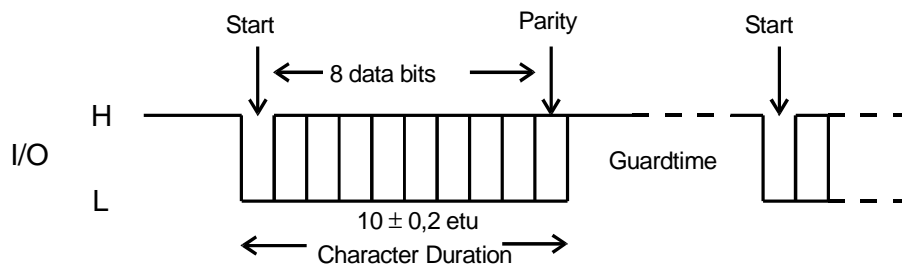
Figure 7.2: Character frame
