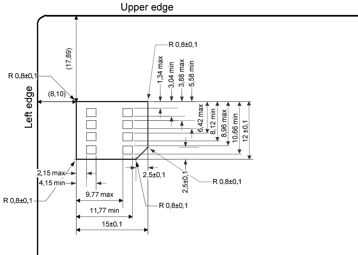
Figure 4.2: Mini-UICC
