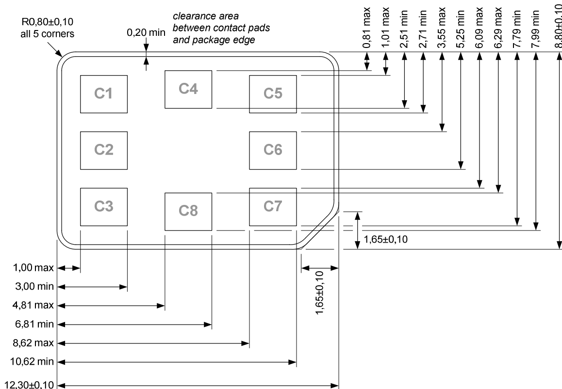
Figure 4.3: 4FF
