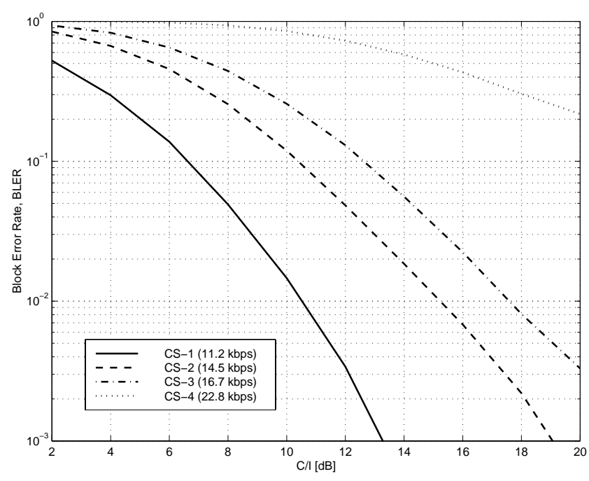
Figure 23: BLER for TU50, no frequency hopping, 1 800 MHz
