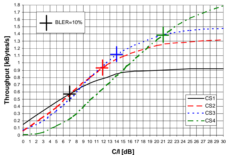
Figure 3: Throughput vs. C/I_c , TU50 ideal FH. Each cross corresponds to a BLER=10%
