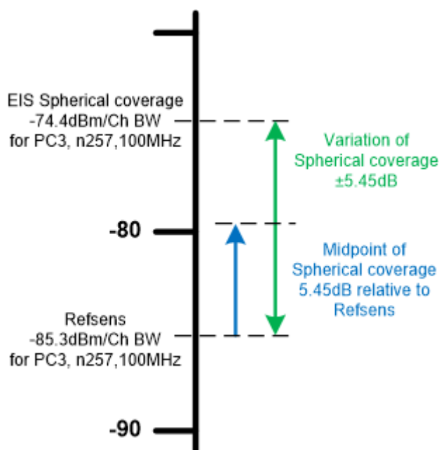
Figure A.2.1.2-1: Example modelling of variation within spherical coverage directions, Fine beams
