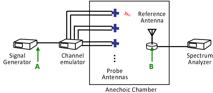
Figure B.3.1-1: Probe Power Calibration Setup
