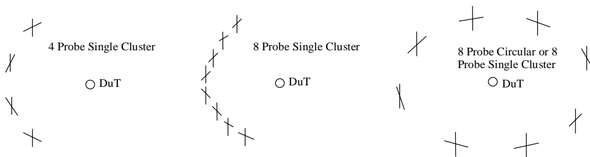
Figure 6.3.1.1.1-1: Some Practical Antenna Probe Configurations, (shown with dual polarization)
