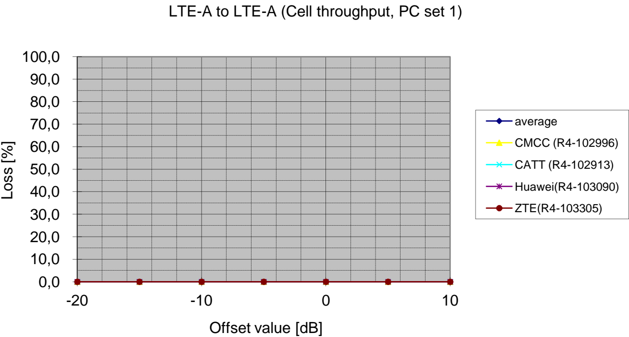
Figure 12.27 average 1.6 MHz UTRA uplink capacity loss (TPC set 1)
