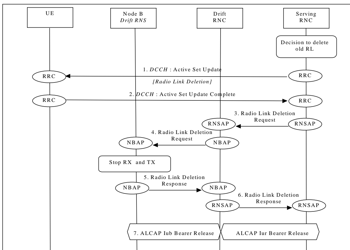
Figure 25: Soft Handover - Radio Link Deletion (Branch Deletion)
