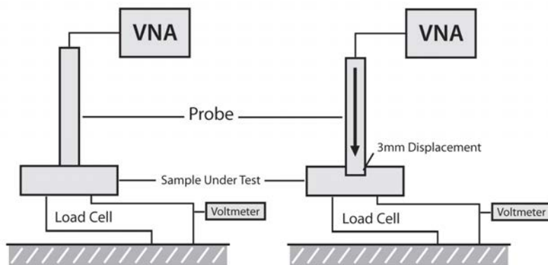
Figure H.1 OCP setup with fixed sensor displacement.
