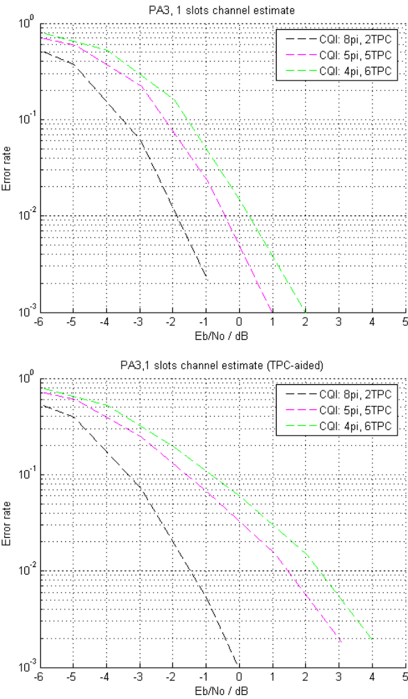
Figure 4.1.2.1-1: CQI performance in PA3, 1 slot channel estimation, with and without TPC-assistance
