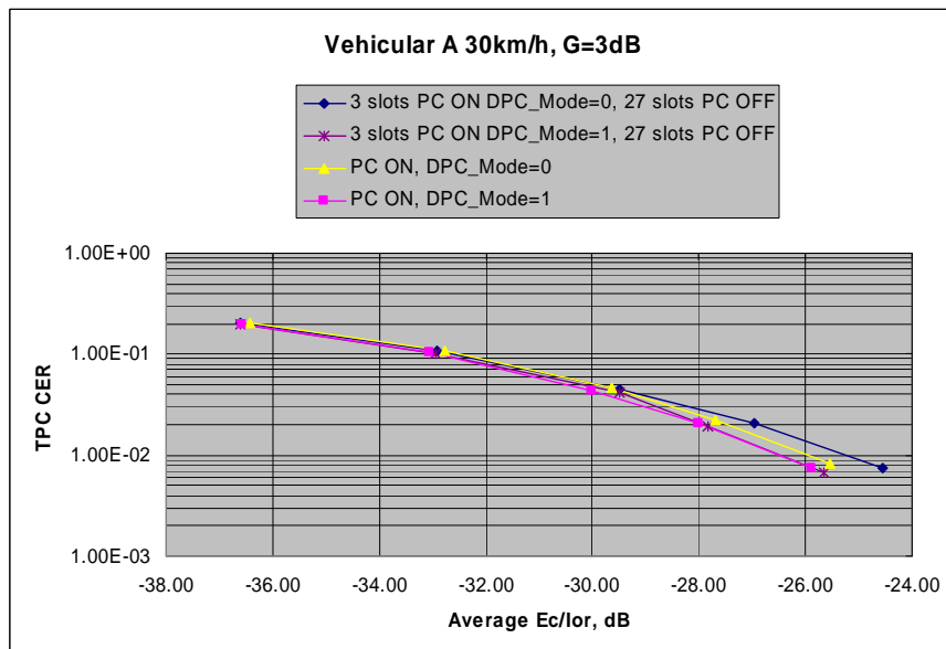
Figure 4.2.2.2-3 F-DPCH performance with different PC modes and discontinuous PC, vehicular A 30km/h, G=3dB.
