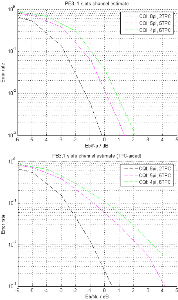
Figure 4.1.2.2.1-3: CQI performance in PB3, 1 slot channel estimation, with and without TPC-assistance
