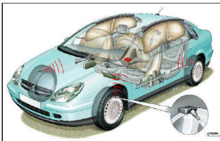
Figure A.10: TPMS Function and implementation
