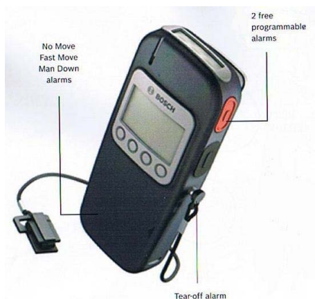
Figure A.8: Portable alarm equipment
