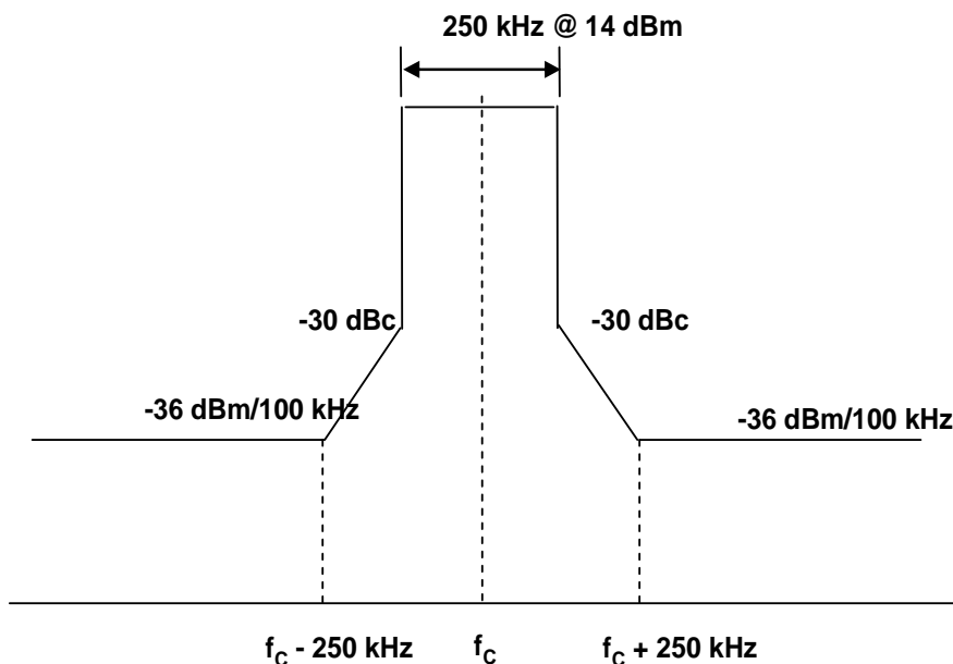
Figure B.3: Metering and Alarms Spectrum Mask
