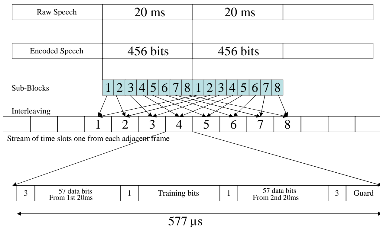
Figure C.1: Generic GSM Frame Structure
