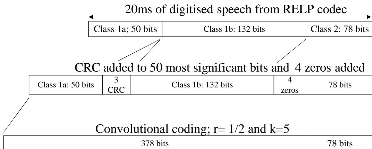
Figure C.2: Full Rate Speech coding
