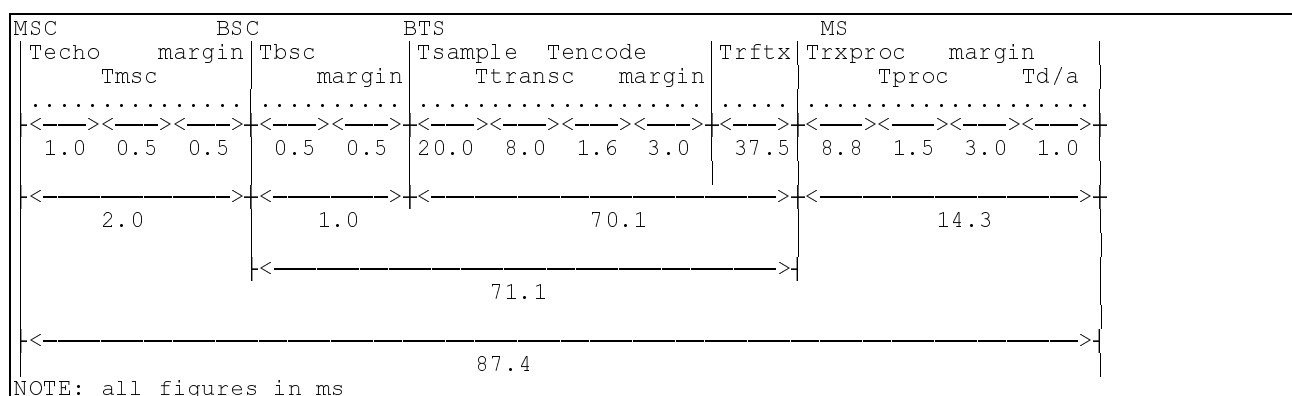
Figure 4/1b: Uplink delay distribution for TCH/FS (16 Kbit/s Abis)
