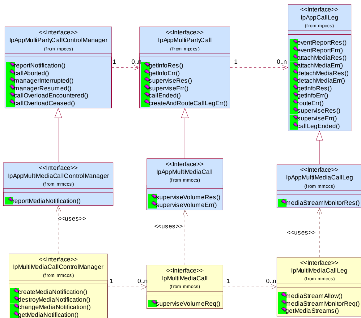
Figure 1: Application Interfaces
