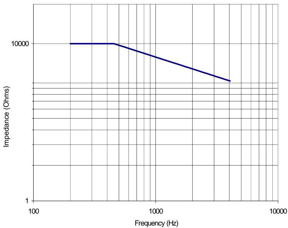
Figure 4: Minimum impedance in the voice band
