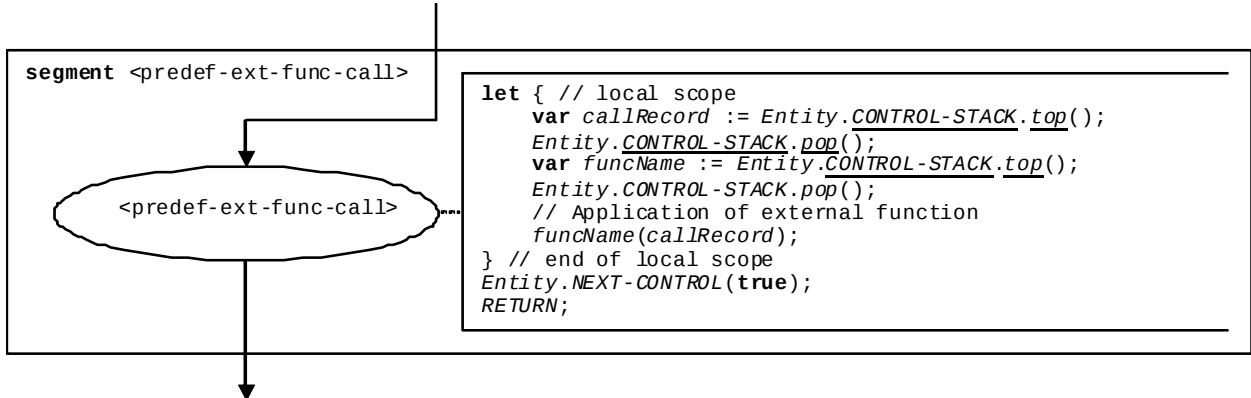
Figure 85: Flow graph segment <predef-ext-func-call>
