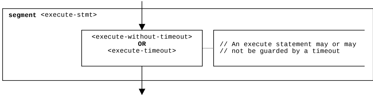
Figure 67: Flow graph segment <execute-stmt>
