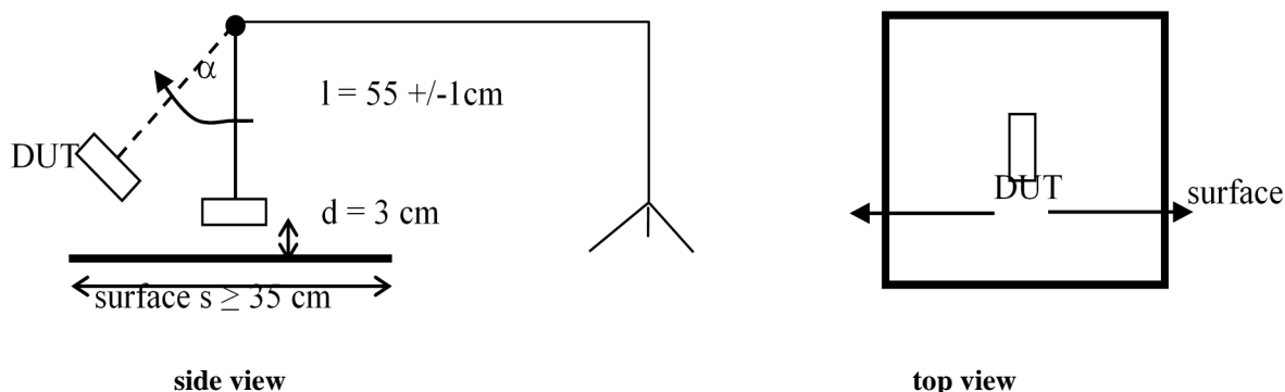
Figure 8: Positioning of handset under test
