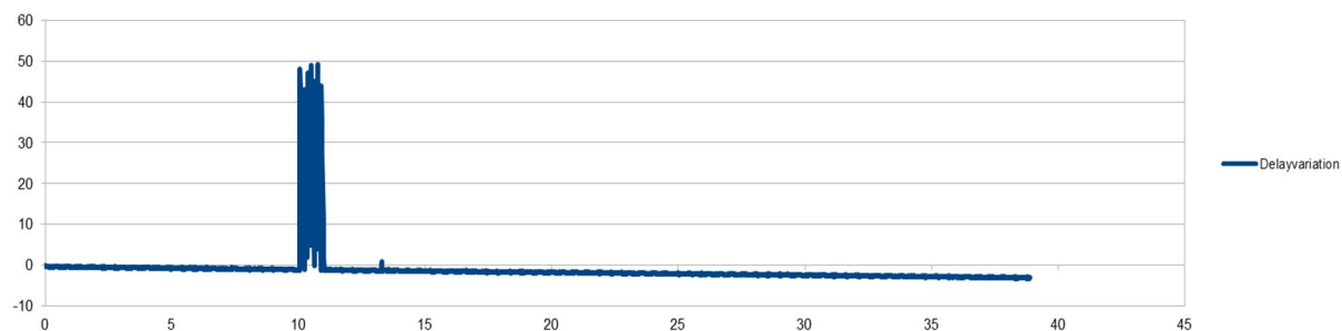
Figure C.1: Example IP delay variation (IPDV) introduced for the measurements shown later in the present document (IPDV in ms vs. time in seconds)
