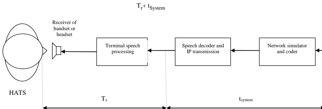
Figure 9: Different blocks contributing to the delay in receive direction
