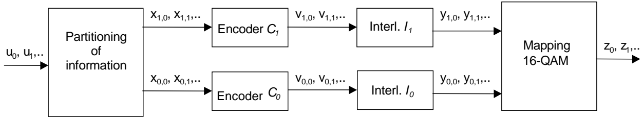
Figure 23: Multilevel coding with 2 levels
