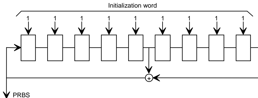
Figure 19: PRBS generator
