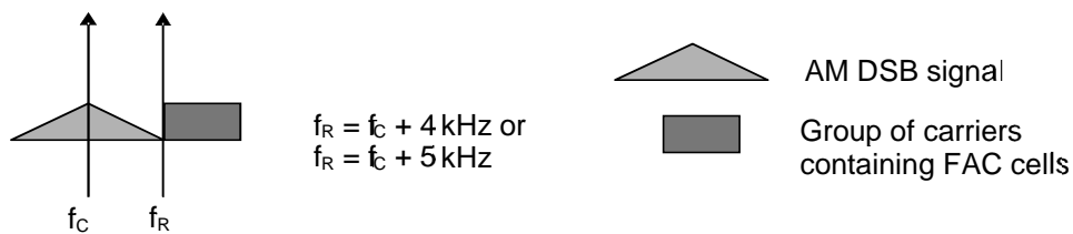
Figure K.2: Example simulcast modes for whole channel offsets
