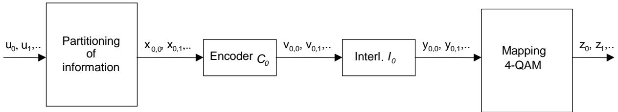
Figure 24: Multilevel coding with 1 level
