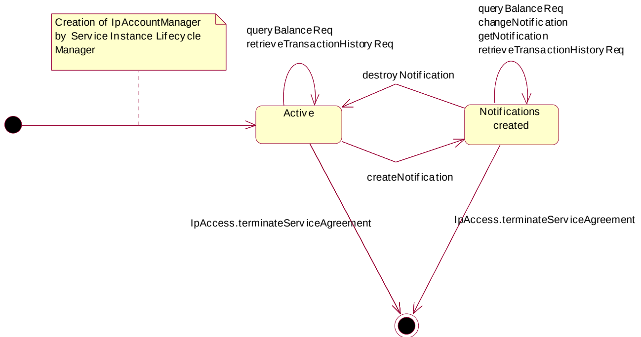
Figure 3: Application view on the IpAccountManager
