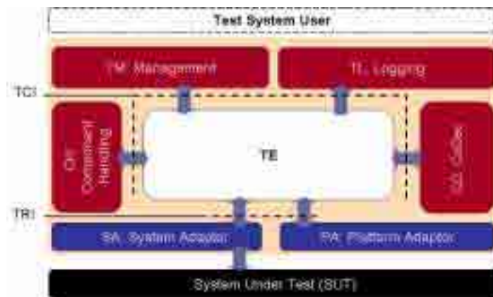
Figure 1: General Structure of a TTCN-3 Test System
