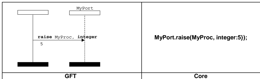
Figure 83: Raise operation with inline template
