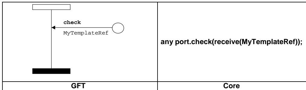
Figure 97: Check a receive on any port
