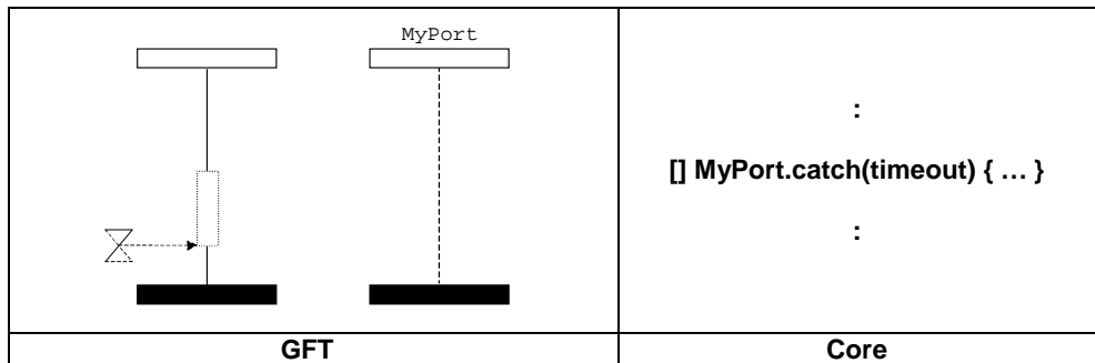
Figure 88: Timeout exception (within a call symbol)
