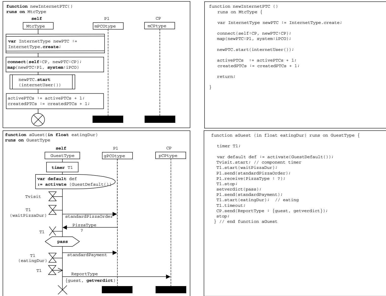
Figure C.2: Restaurant example - newInternetPTC and aGuest functions
