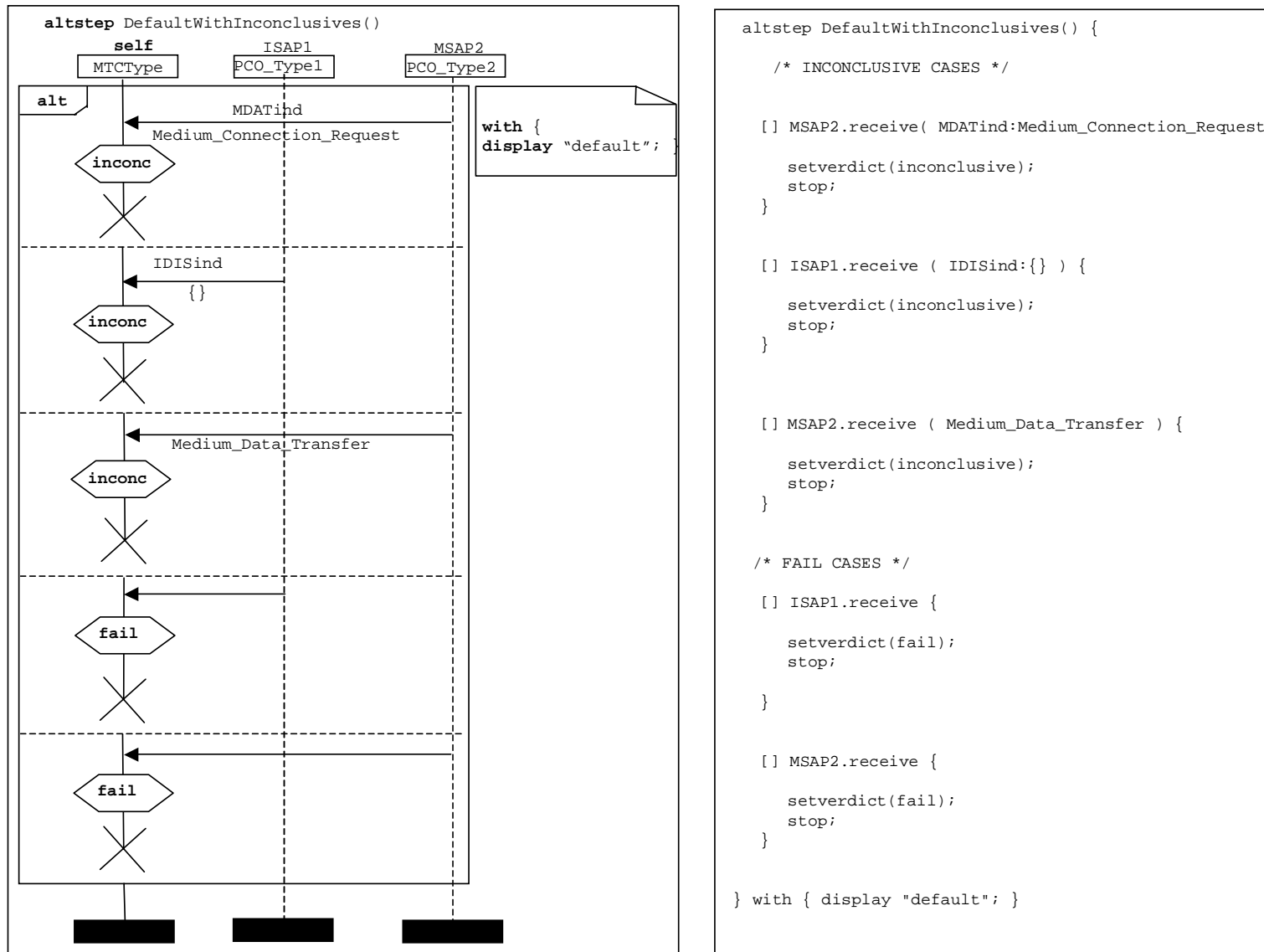
Figure C.14: INRES example - DefaultWithInconclusives altstep
