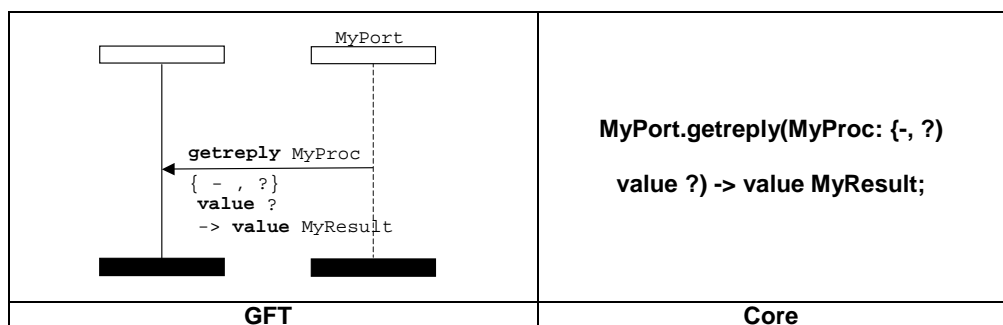
Figure 77: Getreply operation with inline template (outside a call symbol)
