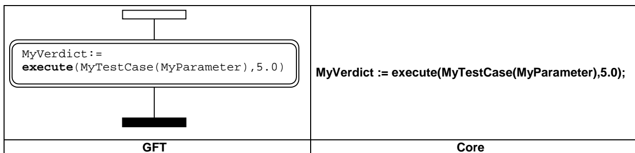
Figure 15: Test case execution
