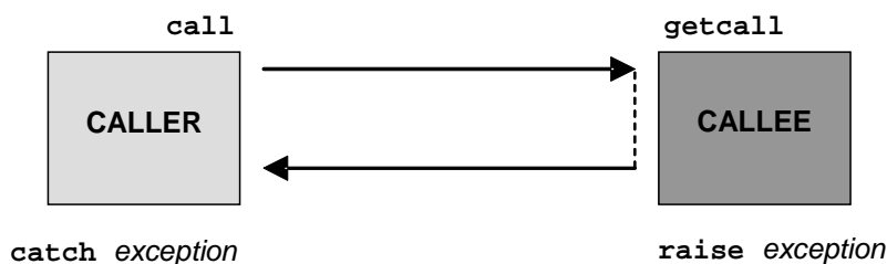
Figure 13: Illustration of non-blocking procedure-based communication
