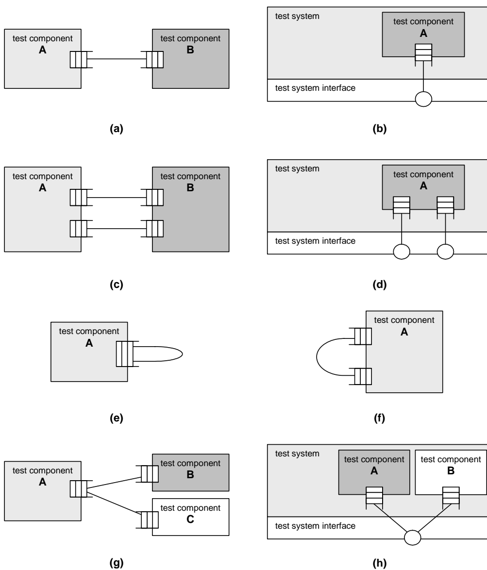
Figure 6: Allowed connections
