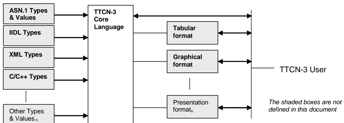
Figure 1: User's view of the core language and the various presentation formats
