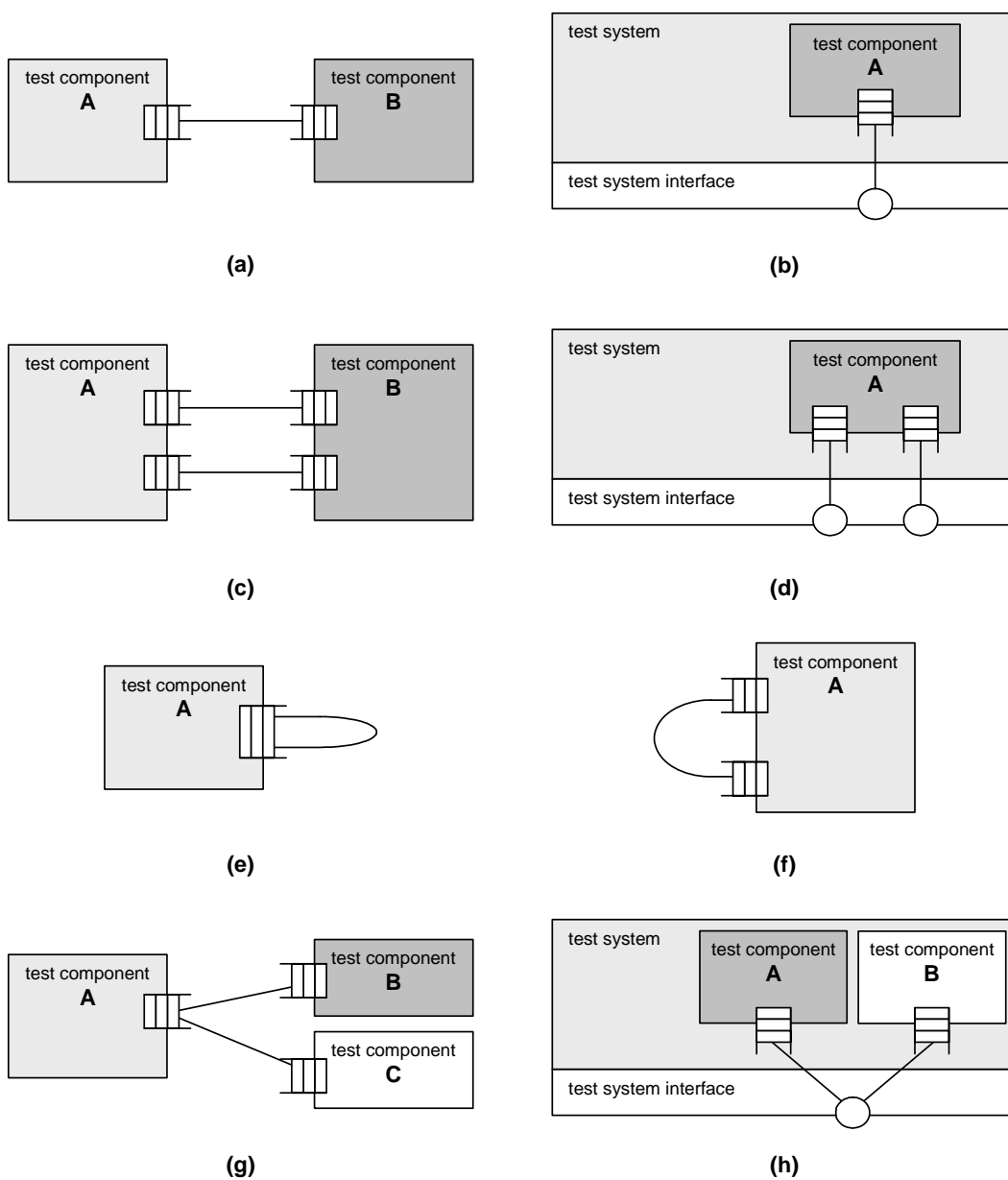
Figure 6: Allowed connections
