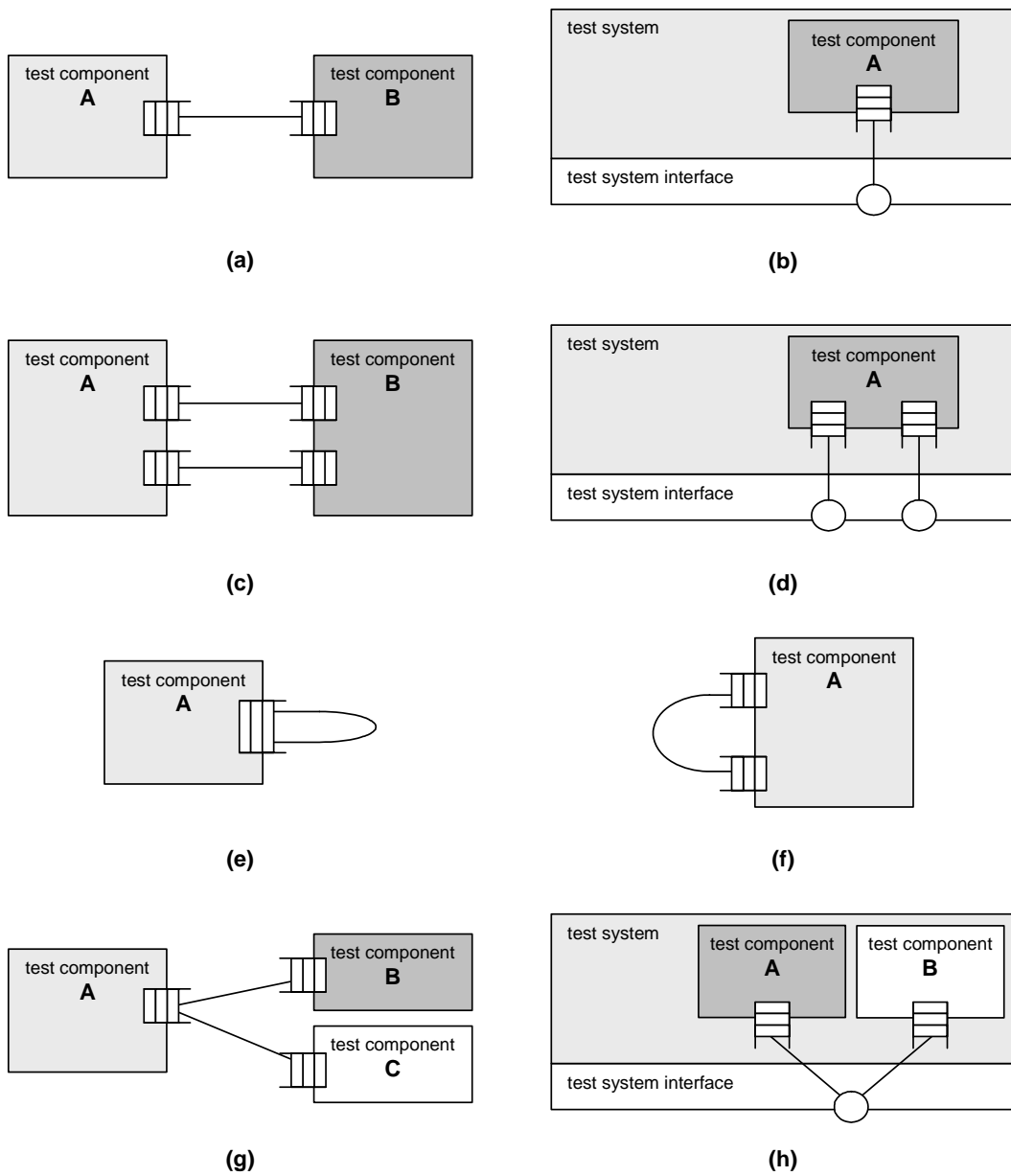
Figure 6: Allowed connections
