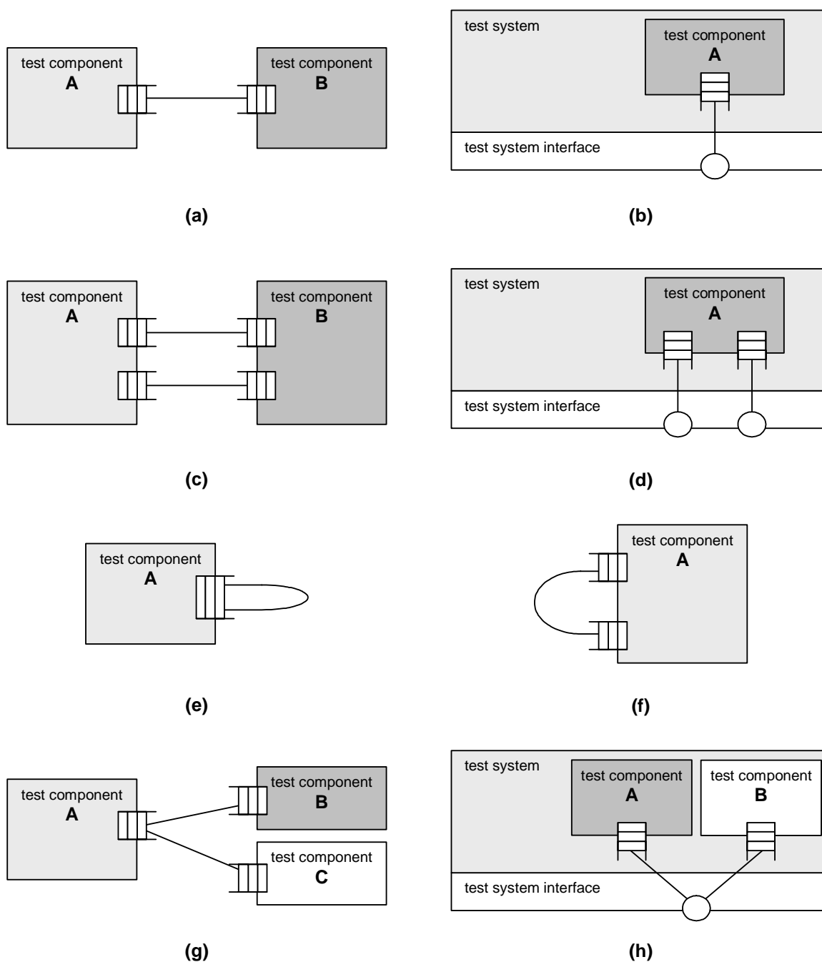
Figure 5: Allowed connections
