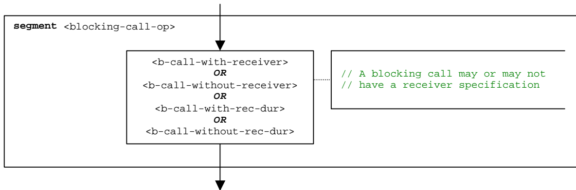
Figure B.31: Flow graph segment <blocking-call-op>
