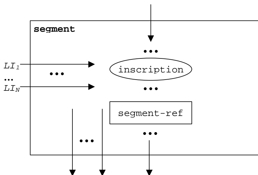
Figure B.8: Schematic flow graph segment description
