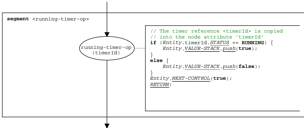
Figure B.105: Flow graph segment <running-timer-op>
