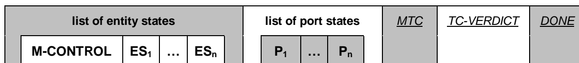
Figure B.12: Structure of a module state
