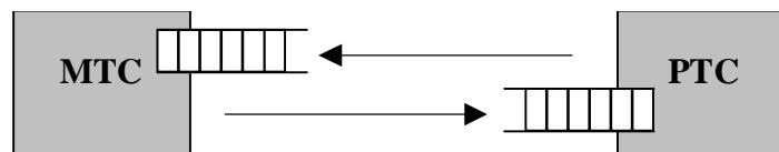
Figure 3: The TTCN-3 communication port model
