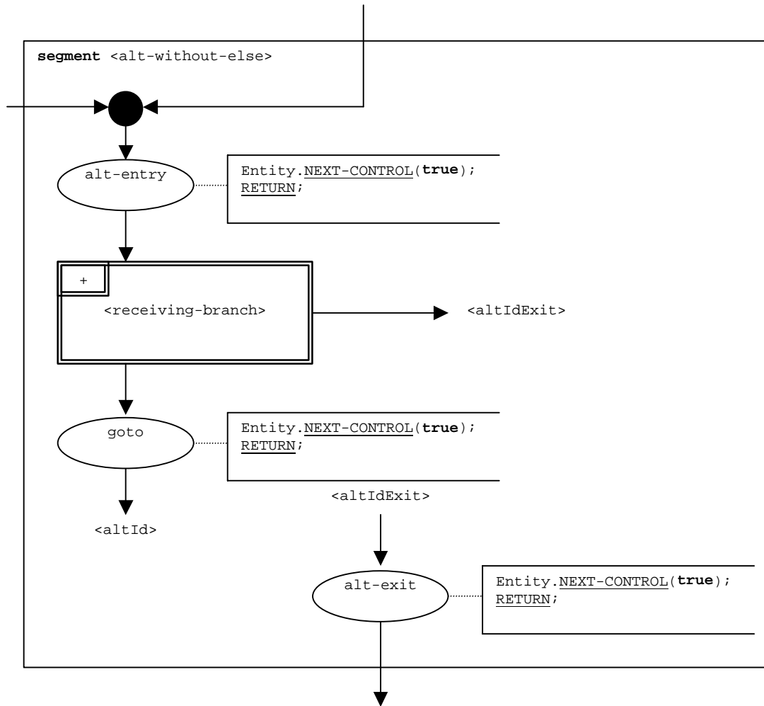
Figure B.27: Flow graph segment &lt;alt-without-else&gt;
