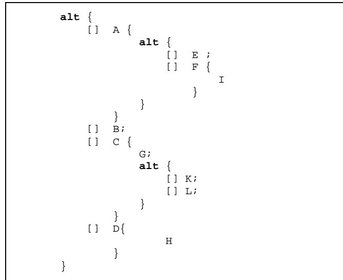
(b) TTCN-3 like representation of (a)
