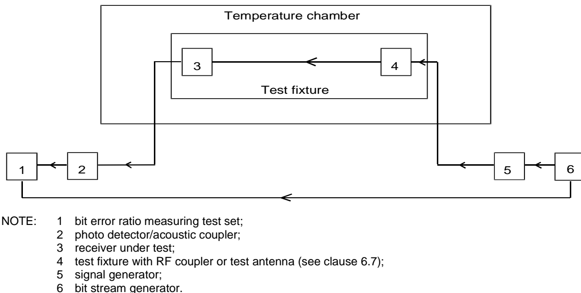
Figure 9: Receiver measurement arrangement for integral antenna (extreme conditions)
