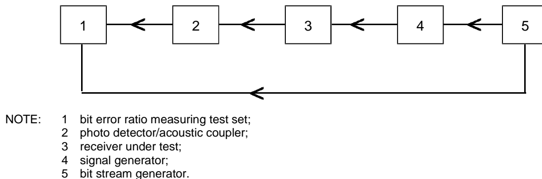
Figure 10: Receiver measurement arrangement for antenna connector
