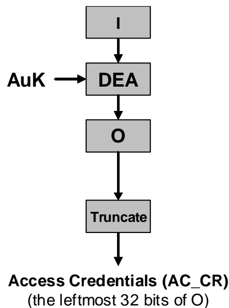
Figure D.2: Access Credentials computation
