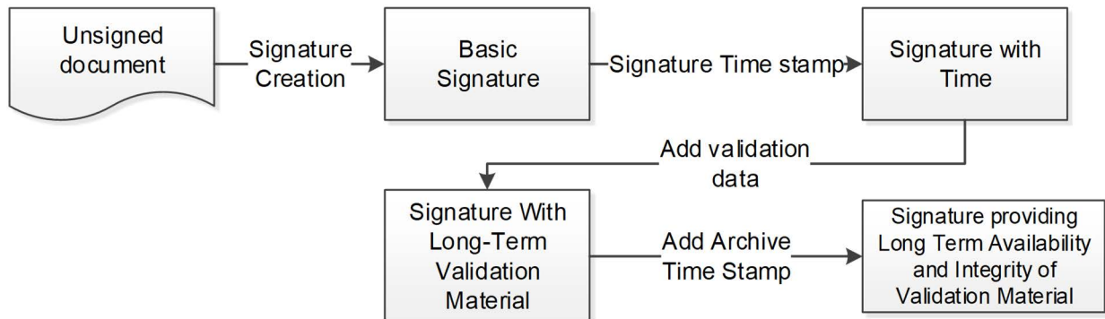
Figure 4: Signature Lifecycle
