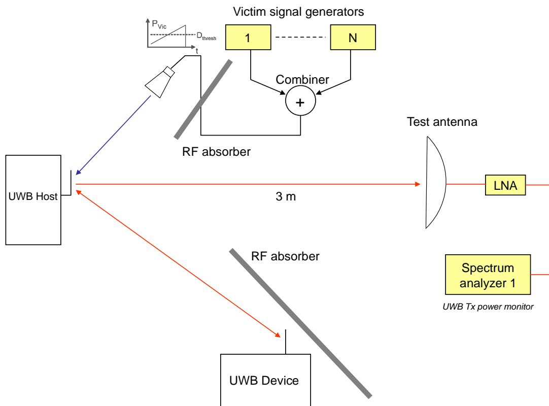
Figure 19: Example Setup for radiated DAA measurements
