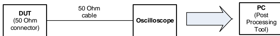
Figure 26: General test setup to execute the time domain procedure for DC measurement in the case of conducted emission
