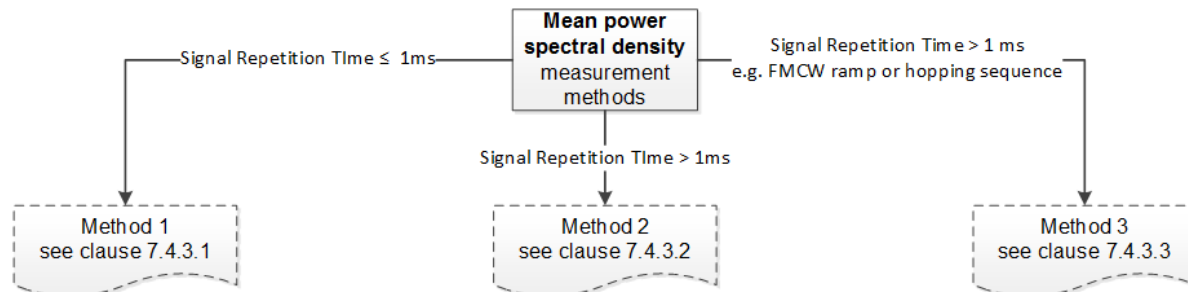
Figure 9: Overview mean power spectral density measurement methods
