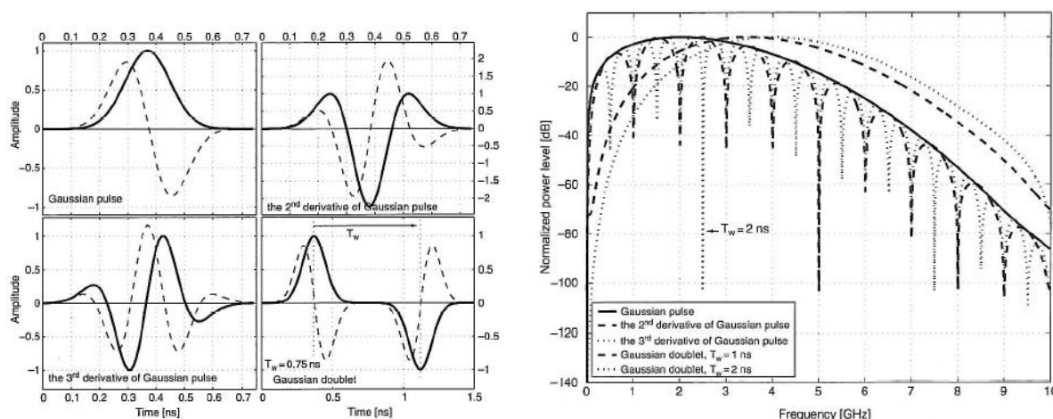
Figure 1: Example of Pulse shapes in time domain and the corresponding spectra
