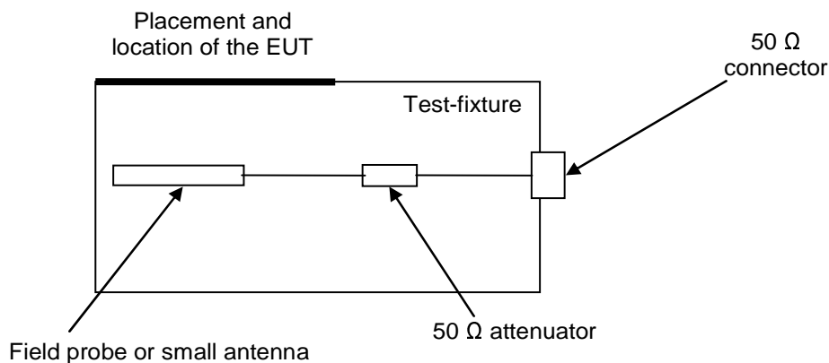
Figure 2: Test fixture
