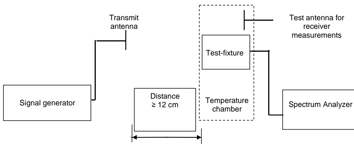
Figure 3: Validation of test set-up without EUT
