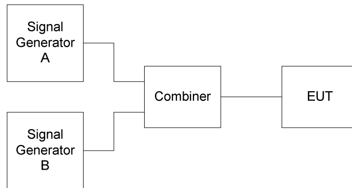
Figure 7: Measurement arrangement
