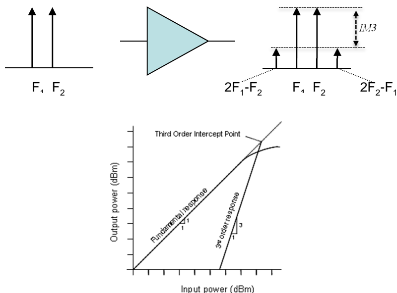
Figure 6: Third order IMD illustration
