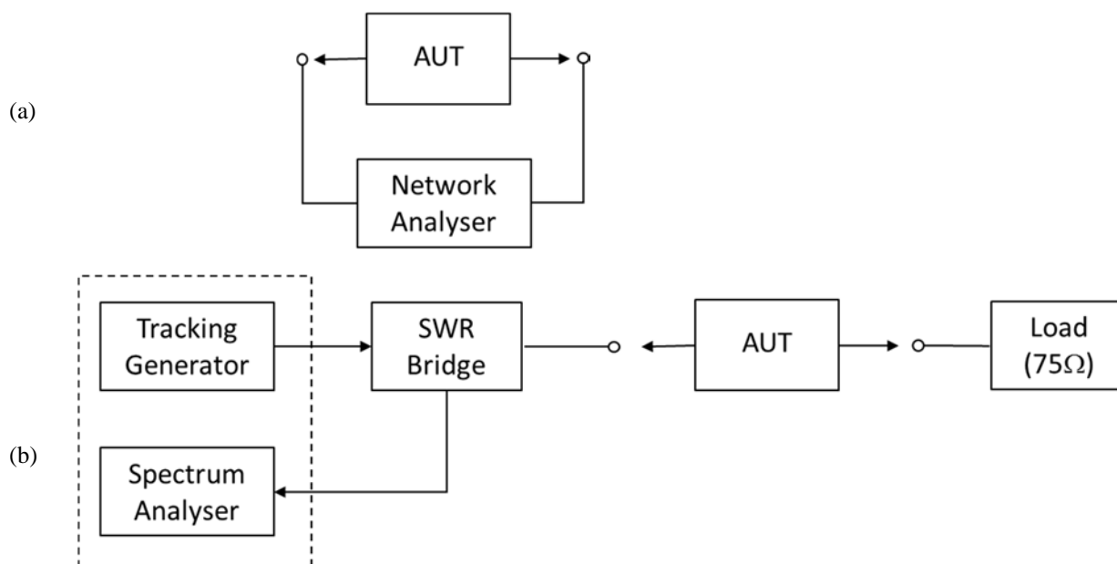
Figure 7: Return loss measurement arrangements using either a network analyser (a) or a spectrum analyser and an external bridge (b)
