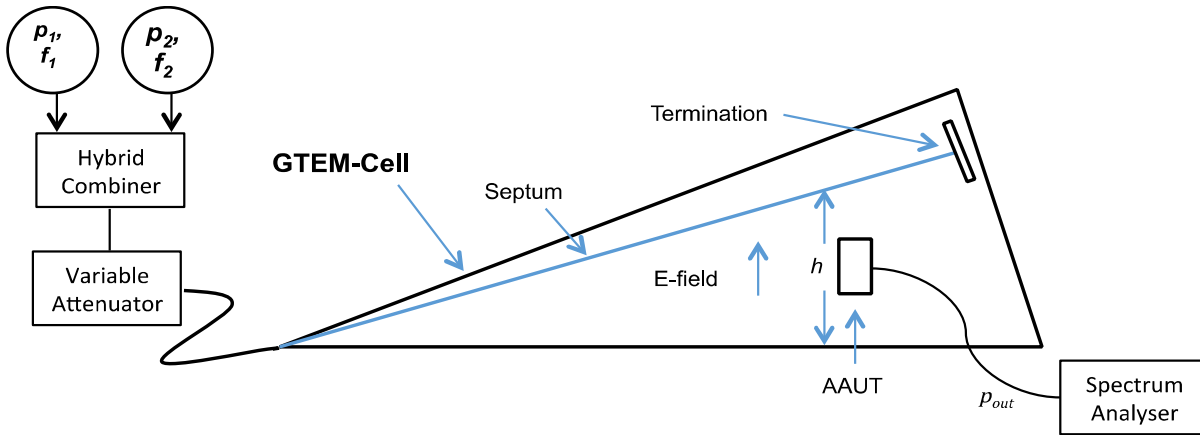
Figure 10: Active antenna intermodulation test arrangement
