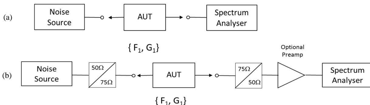
Figure 4: Measurement arrangements for noise figure test
