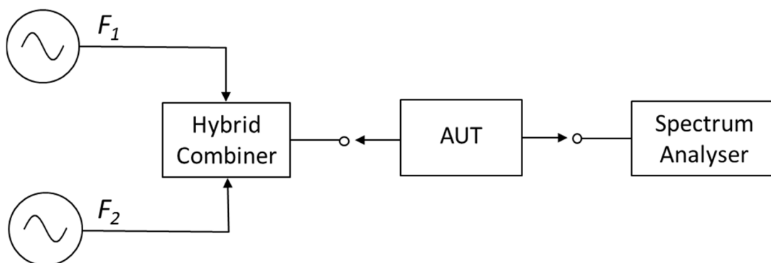
Figure 5: Measurement arrangement for intermodulation test
