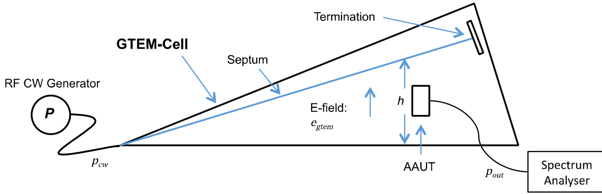
Figure 9: Active antenna gain test arrangement
