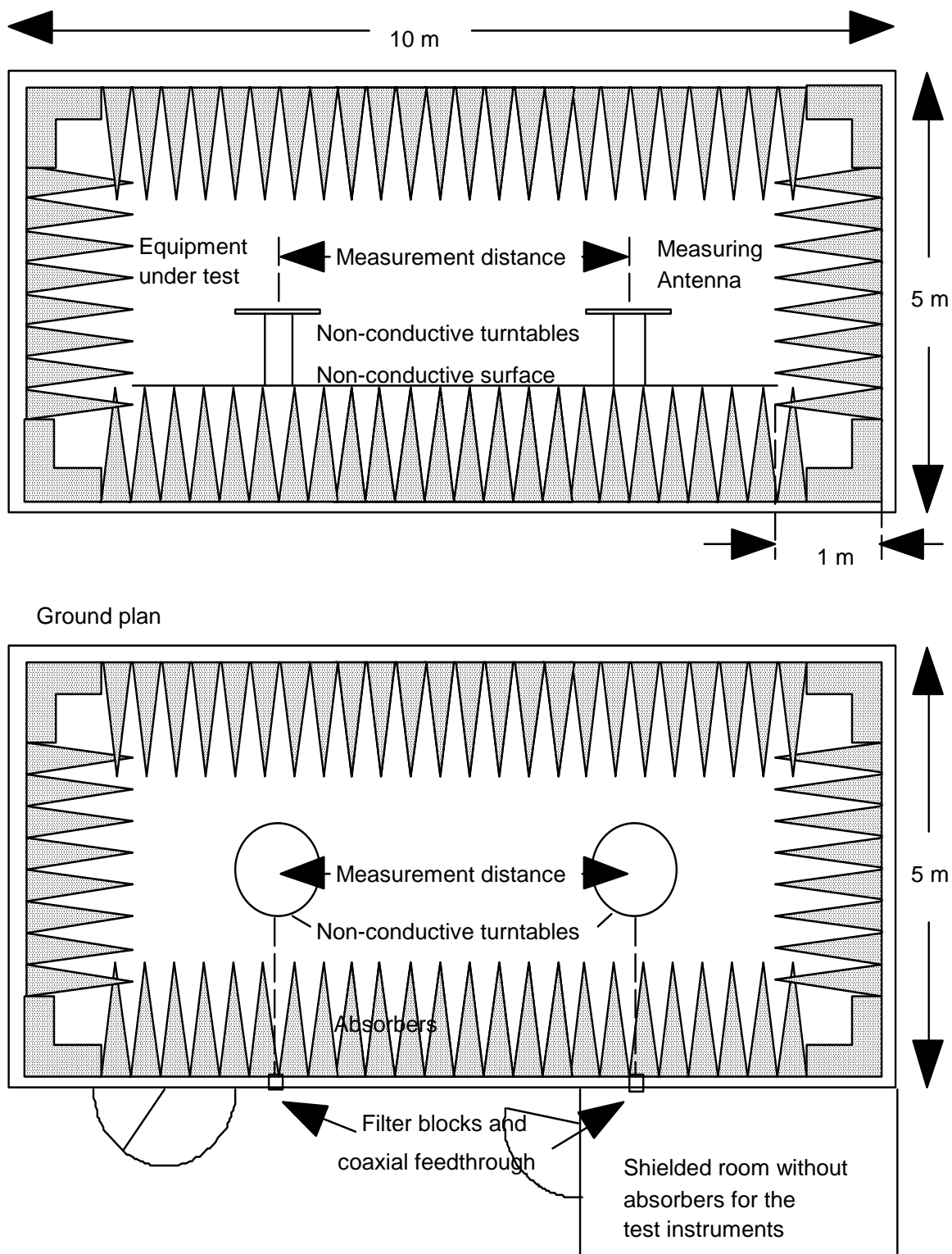
Figure A.3: Example of the construction of an anechoic shielded chamber
