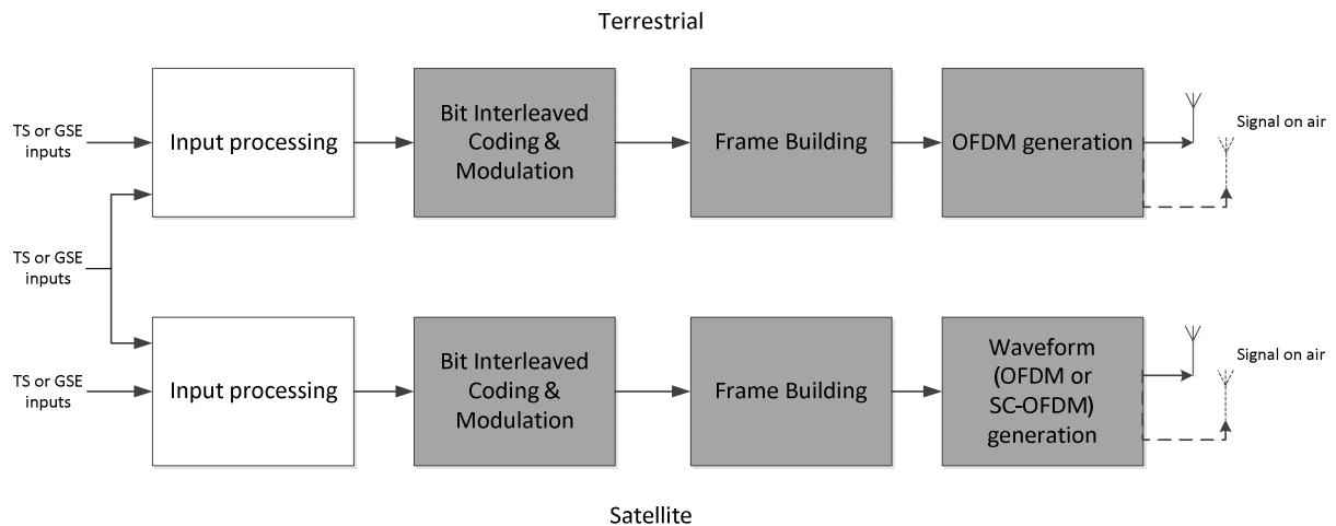
Figure 1: High level NGH physical layer block diagram of the Hybrid Profile - reflected by the present document
