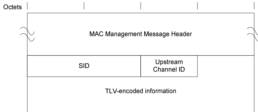
Figure 6-23: Ranging Response
