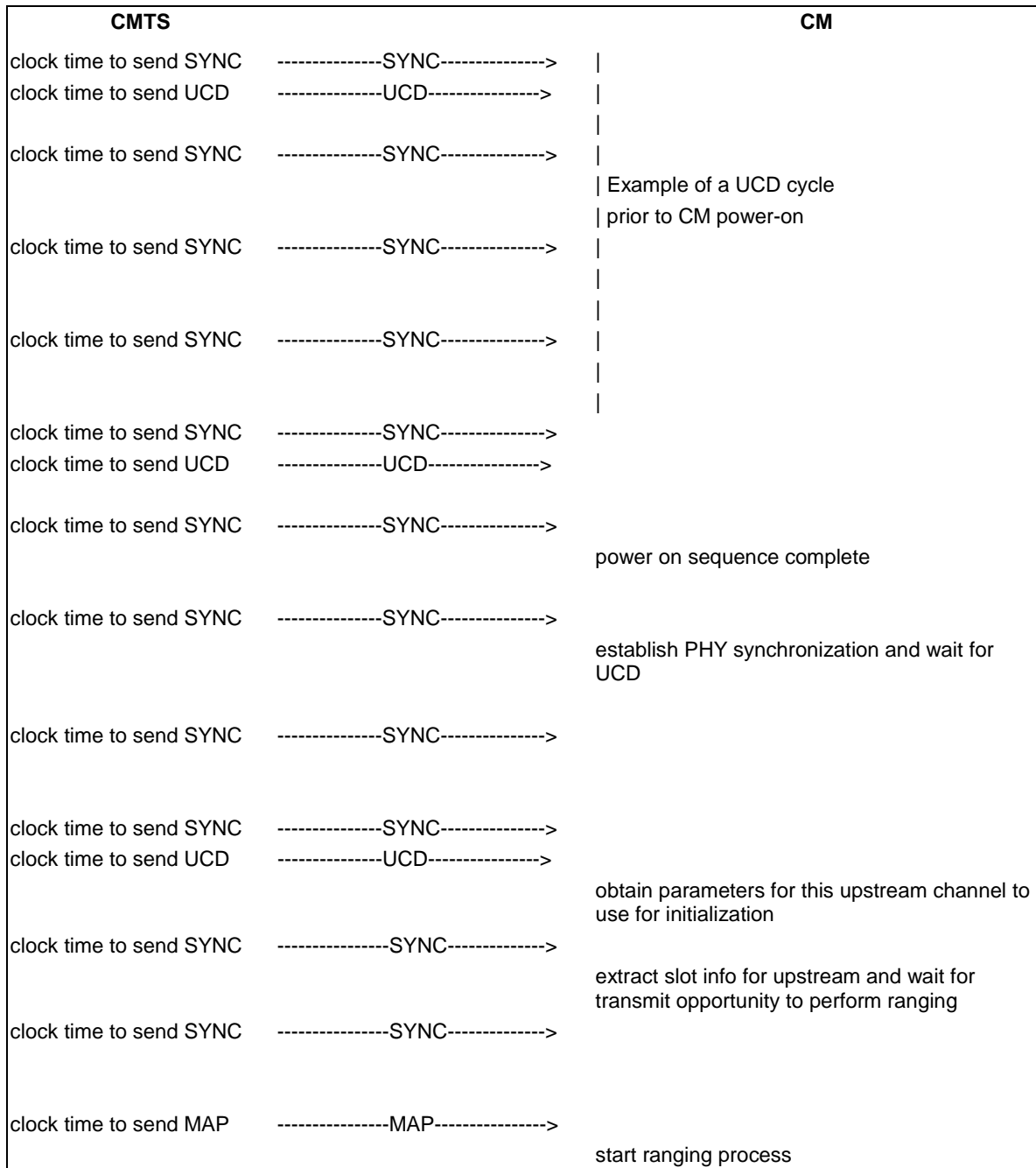
Figure 10-10: Message Flows During Scanning and Upstream Parameter Acquisition
