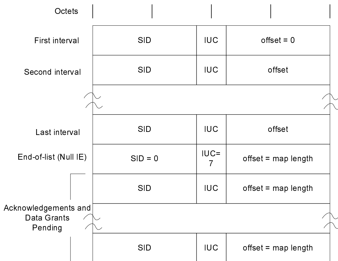
Figure 6-19: MAP Information Element Structure
