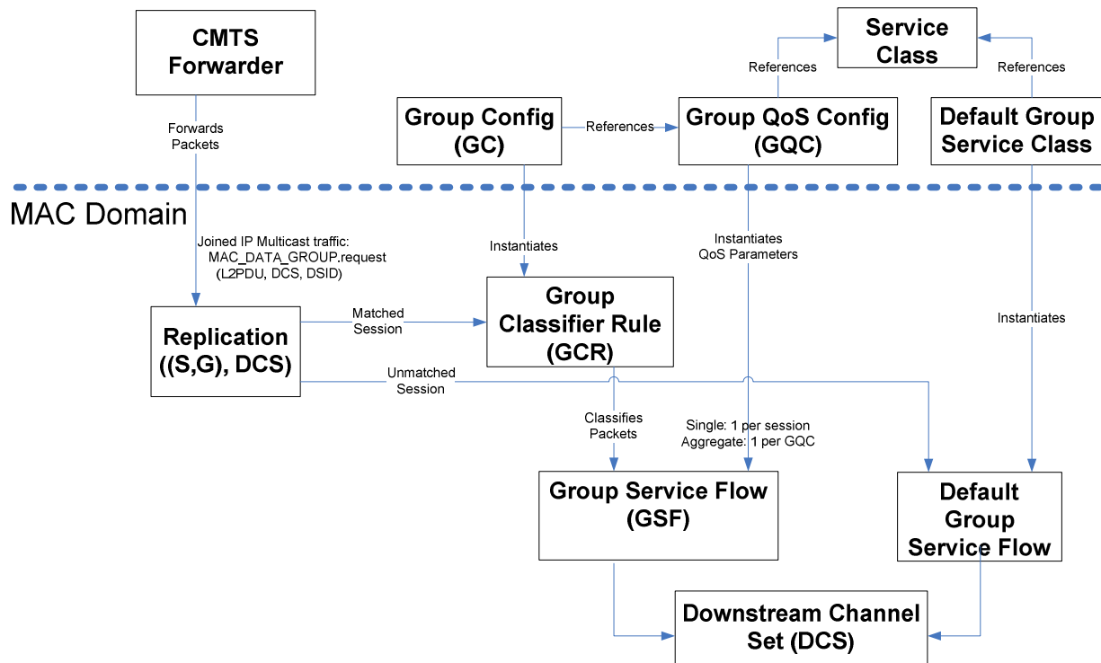
Figure 7-17: IP Multicast QoS Object Model Diagram
