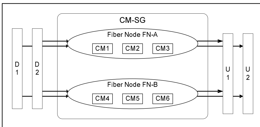
Figure 5-7: Multiple fibre nodes per CM-SG
