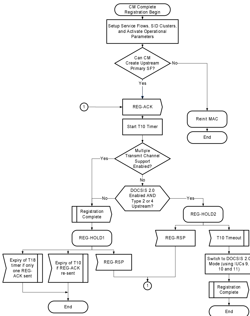
Figure 10-30: CM Completes Registration
