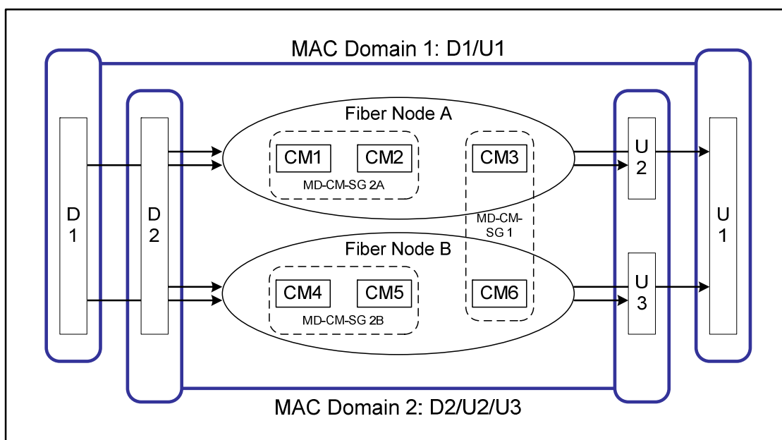
Figure 5-9: Multiple MAC Domains per Fibre Node
