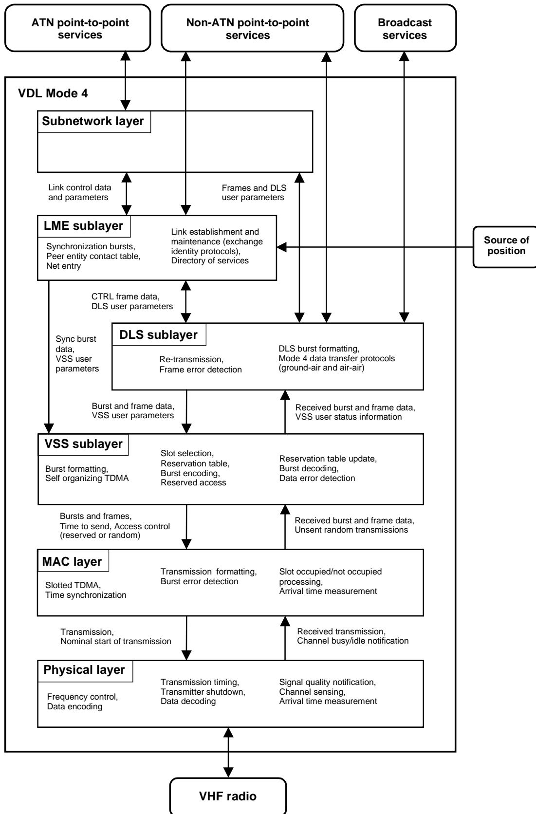
Figure 4.1: Layered structure of VDL Mode 4
