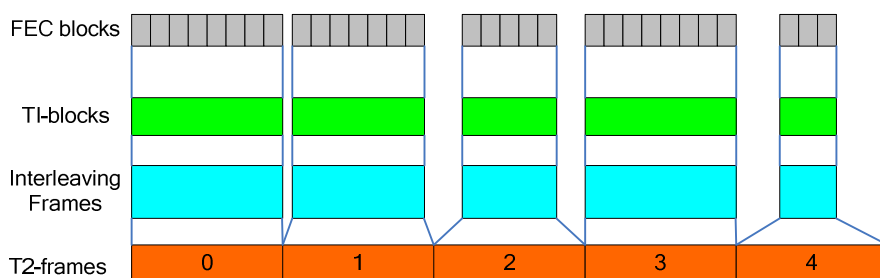
Figure 18(a): Time interleaving for P_1=1 , I_{\text{JUMP}}=1 , N_{\text{TI}}=1
