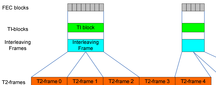
Figure 18(b): Time interleaving for P_1=2 , I_{\text{JUMP}}=2 , N_{\text{TI}}=1
