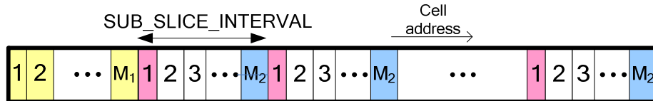
Figure 45: Scheduled data PLPs for T2-frame
