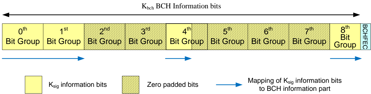
Figure 32: Example of Shortening of BCH information part
