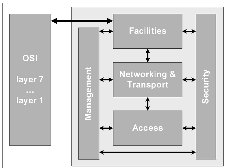
Figure 9: ITS-S gateway
