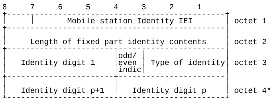
Figure 10.5/GSM 04.xx Mobile station Identity information element
