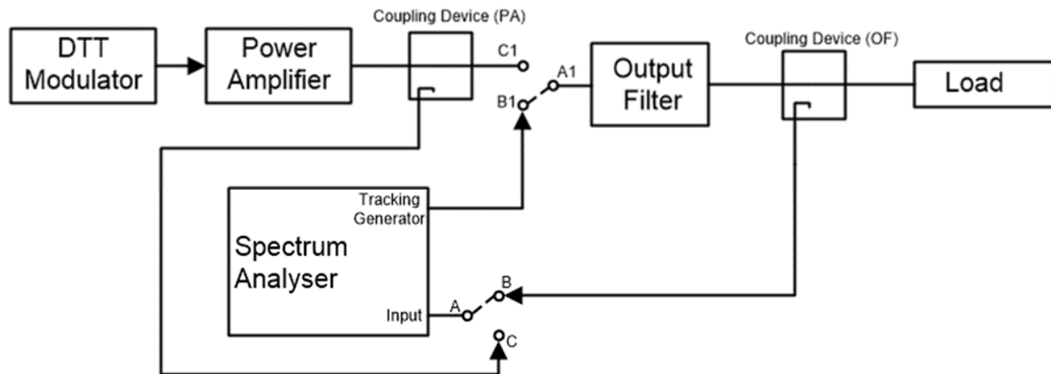
Figure D.1: Practical arrangement for measuring the response of the Output Filter
