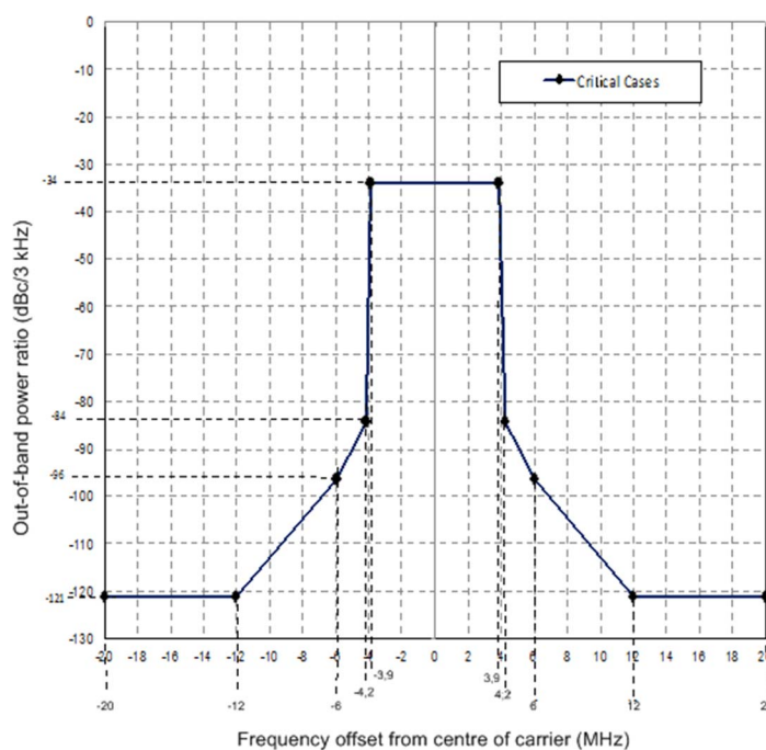
Figure 4.6: Out-of-band limits for transmitter classification H1 using 8 MHz channels
